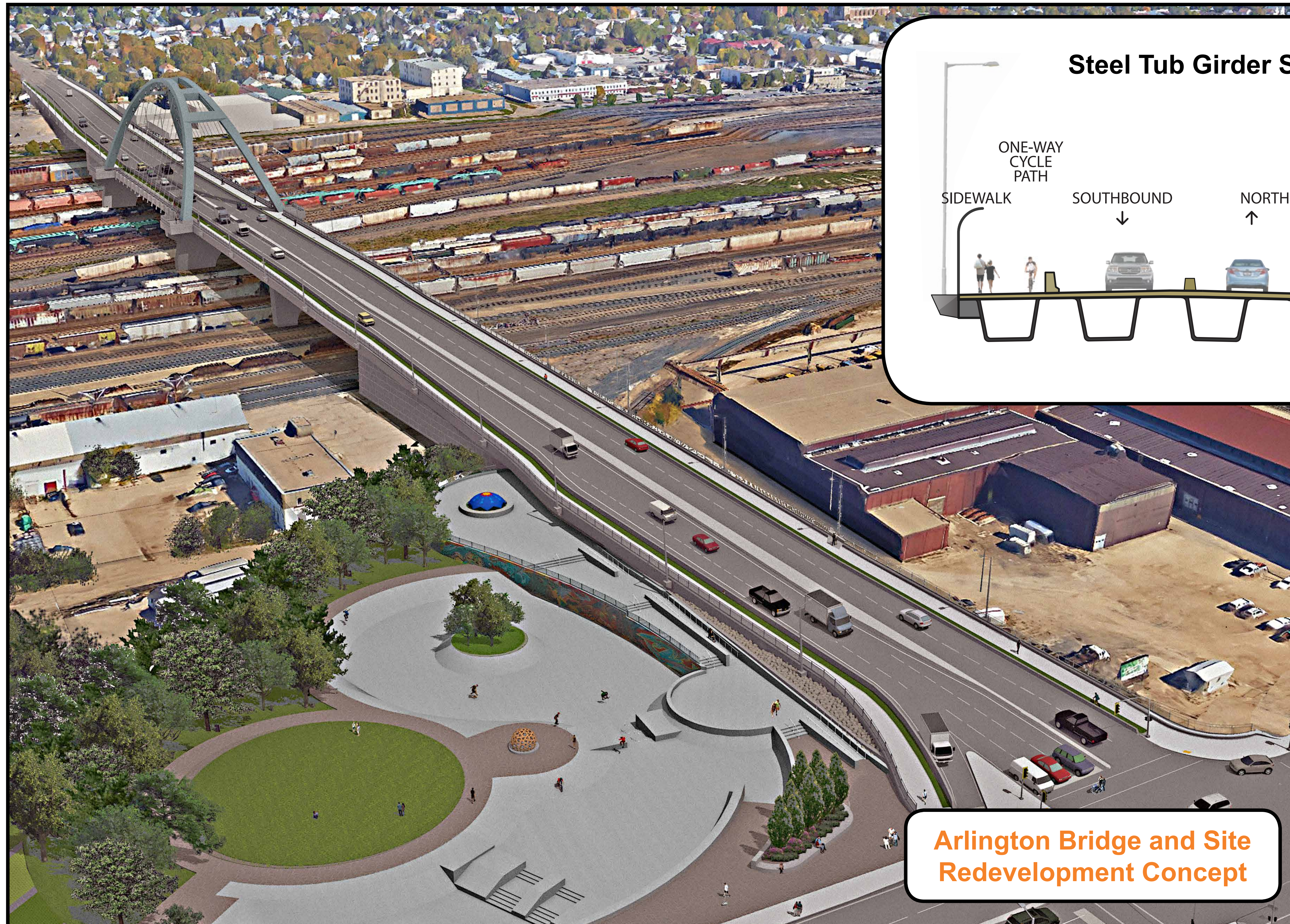
Arlington Bridge Concept
