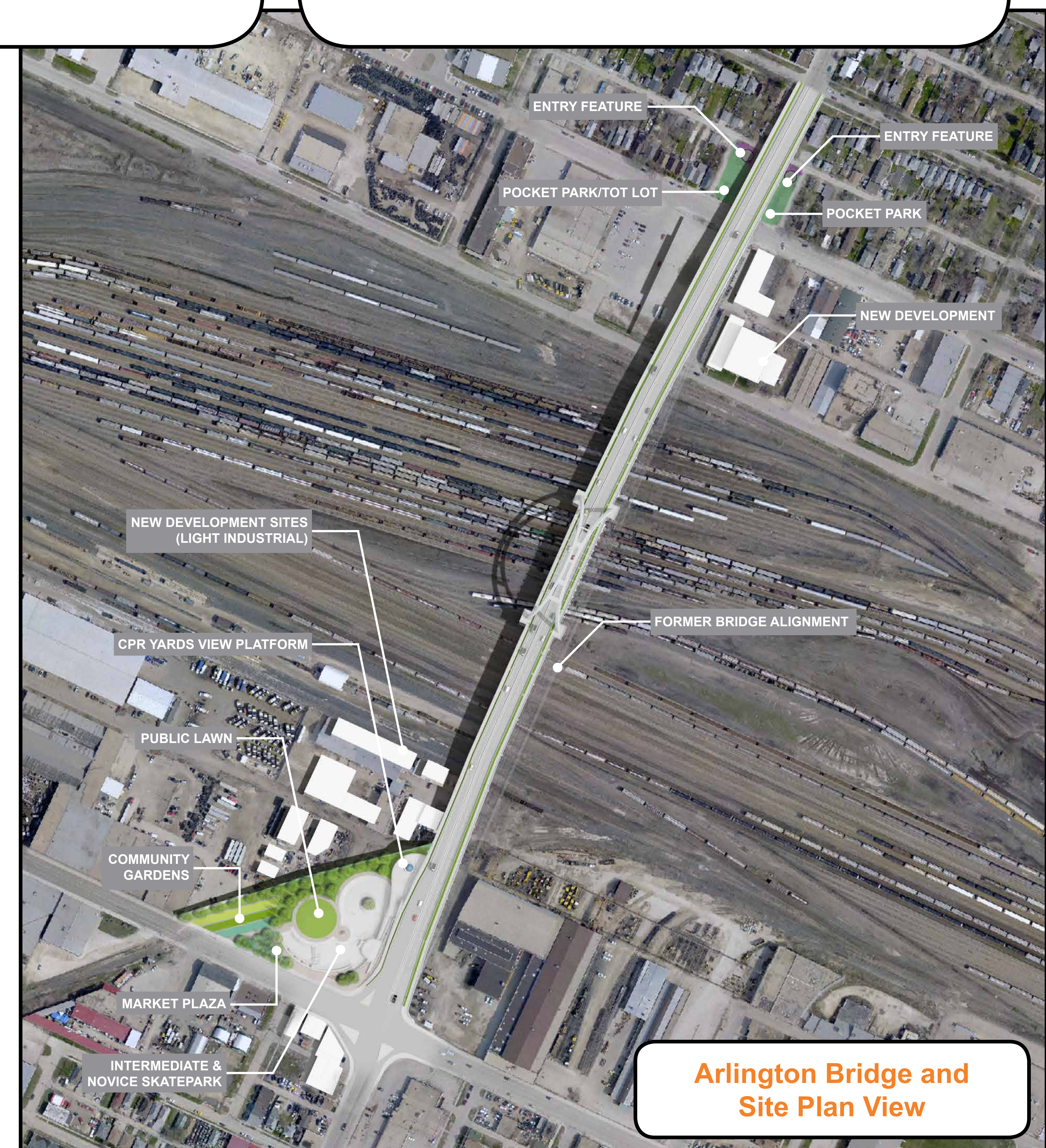
Arlington Bridge and Site Redevelopment Concept
