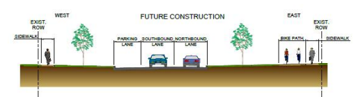
TYPICAL SECTION OF MOLSON STREET KIMBERLY AVENUE TO GRASSIE BOULEVARD
