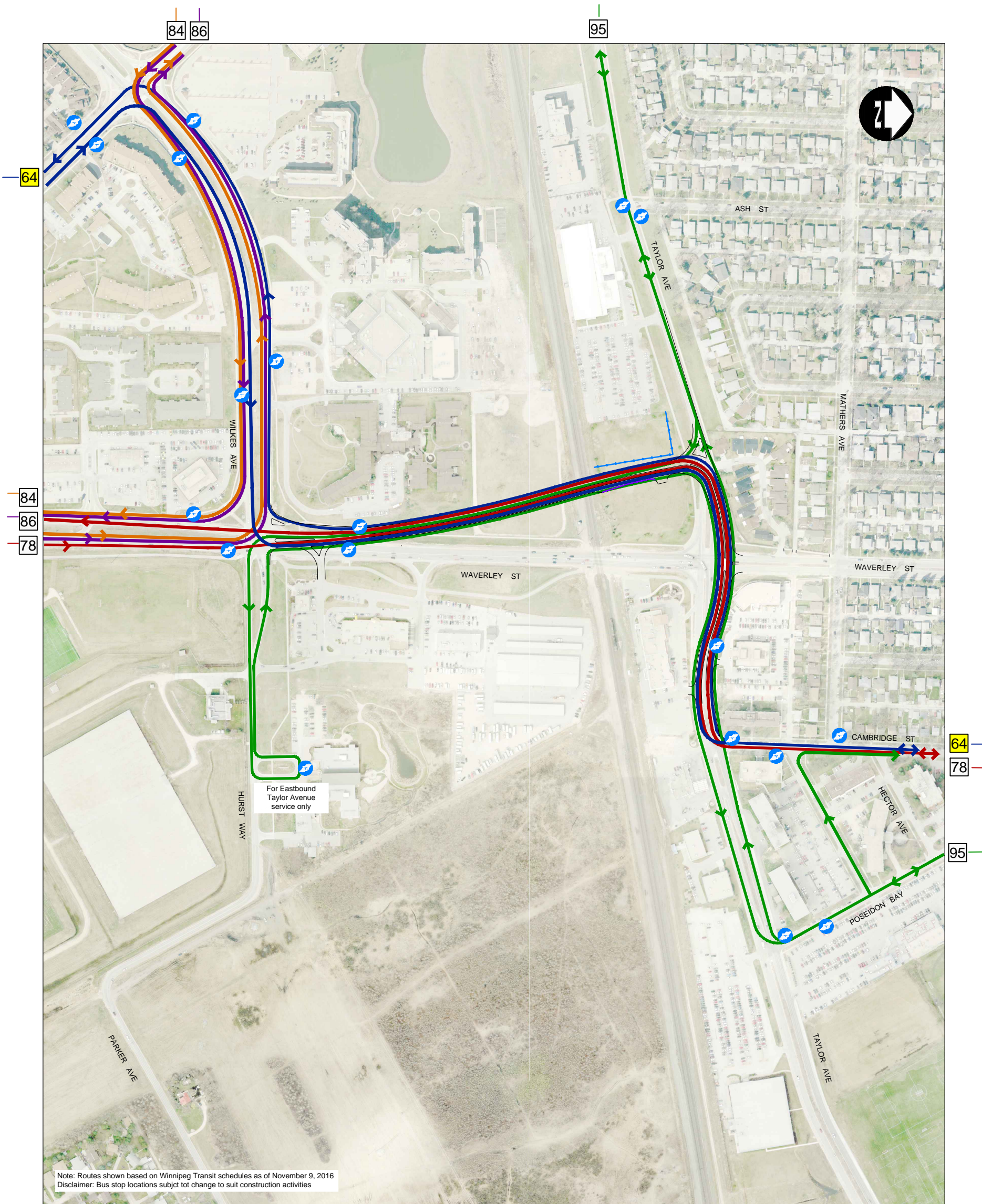
FIGURE 2: TRANSIT ROUTES AND STOPS DURING CONSTRUCTION
