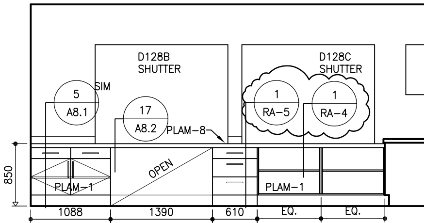
35 CANTEEN 128 A-7.1 SCALE: 1:50 REVISED DRAWING
