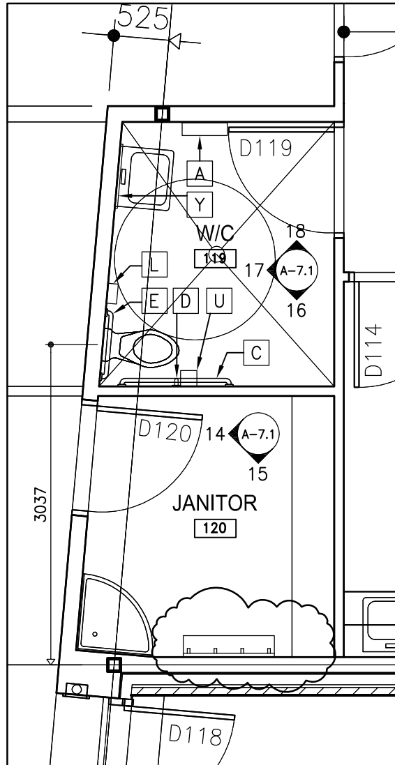
7 JANITOR 120 & WC 119 DETAIL PLAN A-7.1 SCALE: 1:50 REVISED DRAWING
