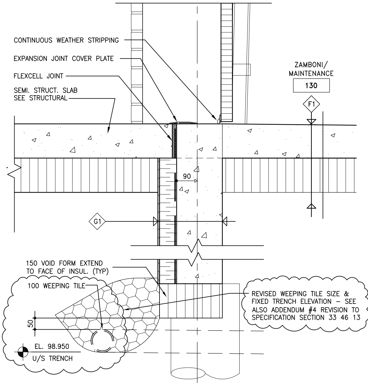
3 WALL SECTION A-4.6 SCALE: 1:10 REVISED DRAWING
