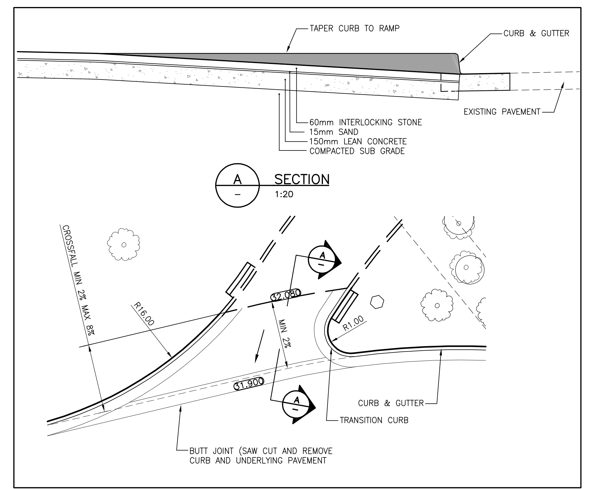
1 ENTRANCE RAMP DETAIL 1:100
