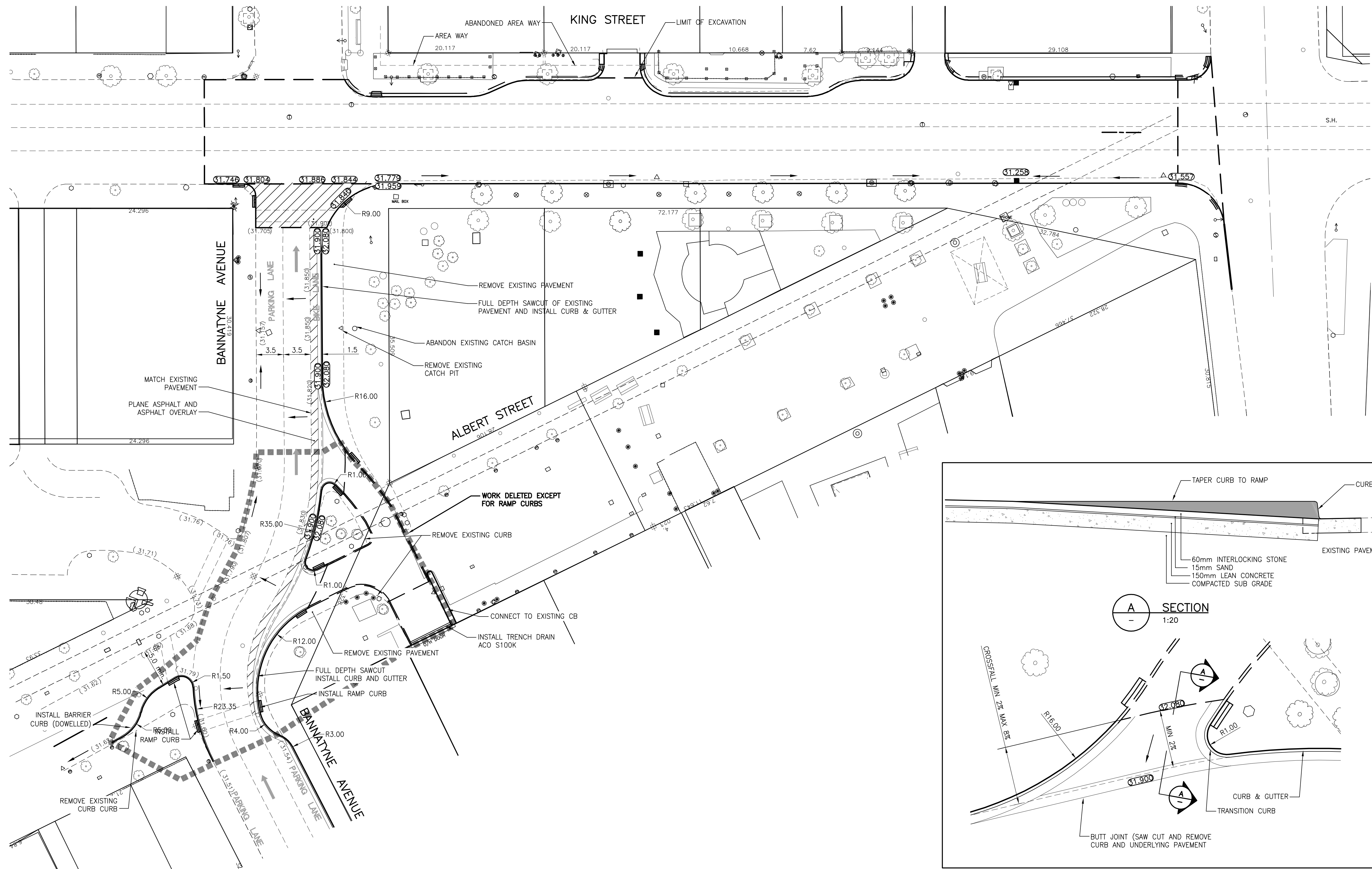
1 ENTRANCE RAMP DETAIL 1:100
