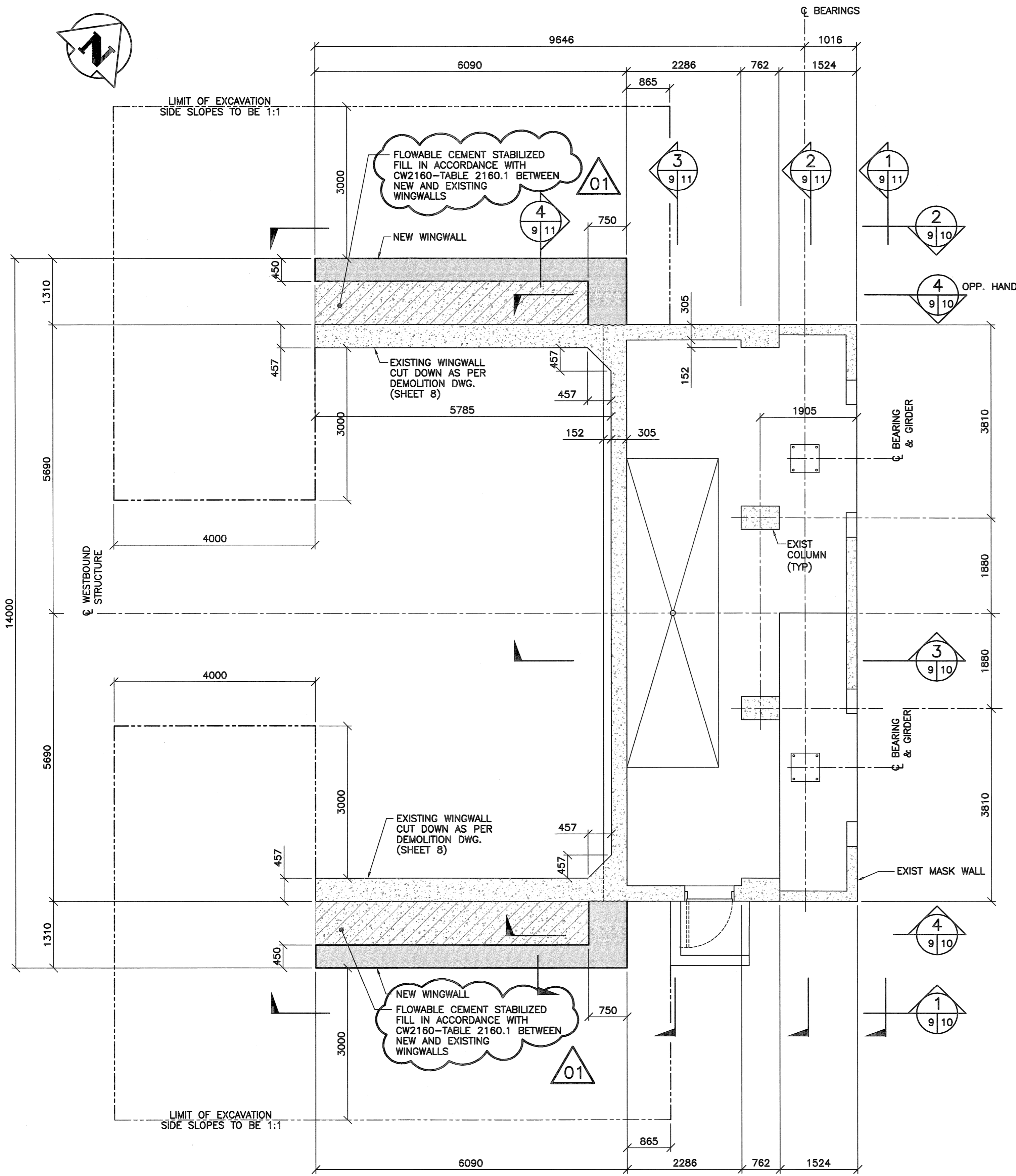
1 LOWER LEVEL PLAN 1 : 50
