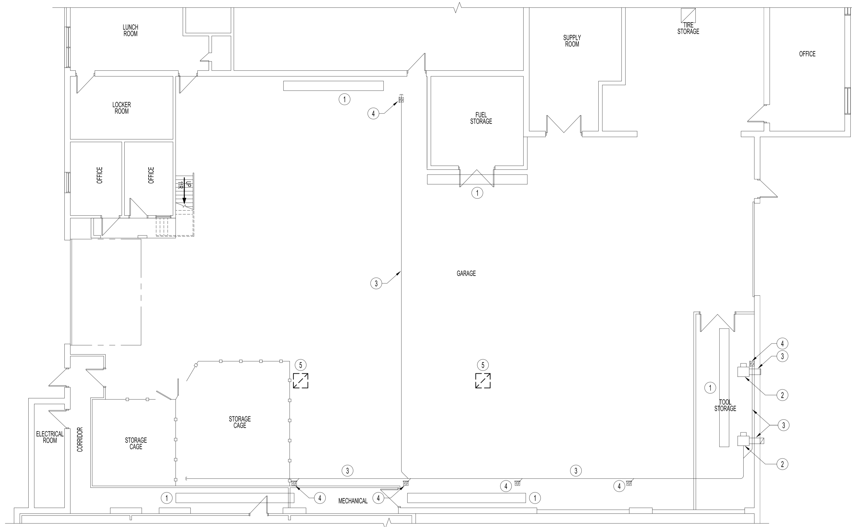
PARTIAL MAIN FLOOR PLAN - MECHANICAL DEMOLITION SCALE: 1/8" = 1'-0"
