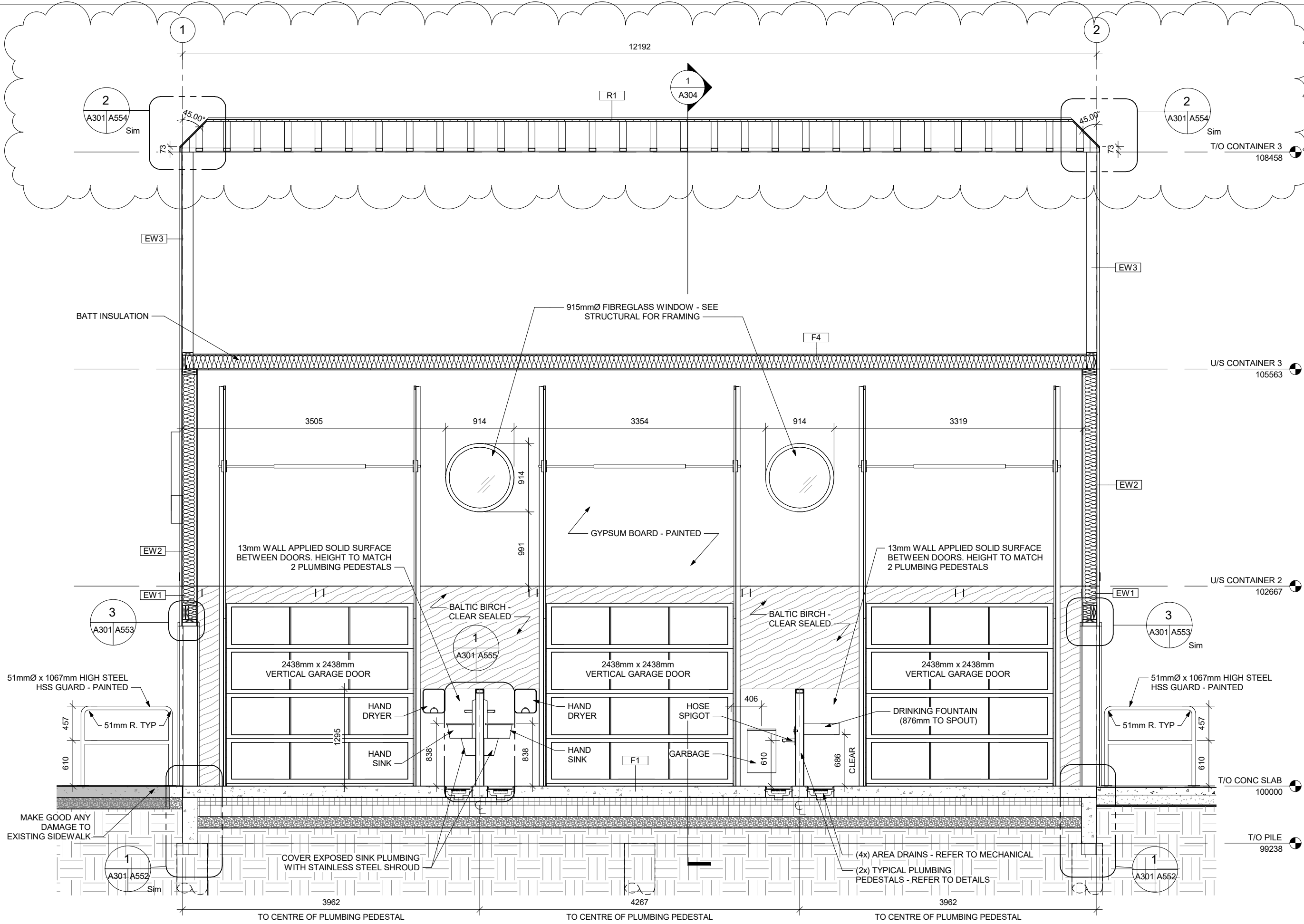
1 BUILDING SECTION 1 1:48
