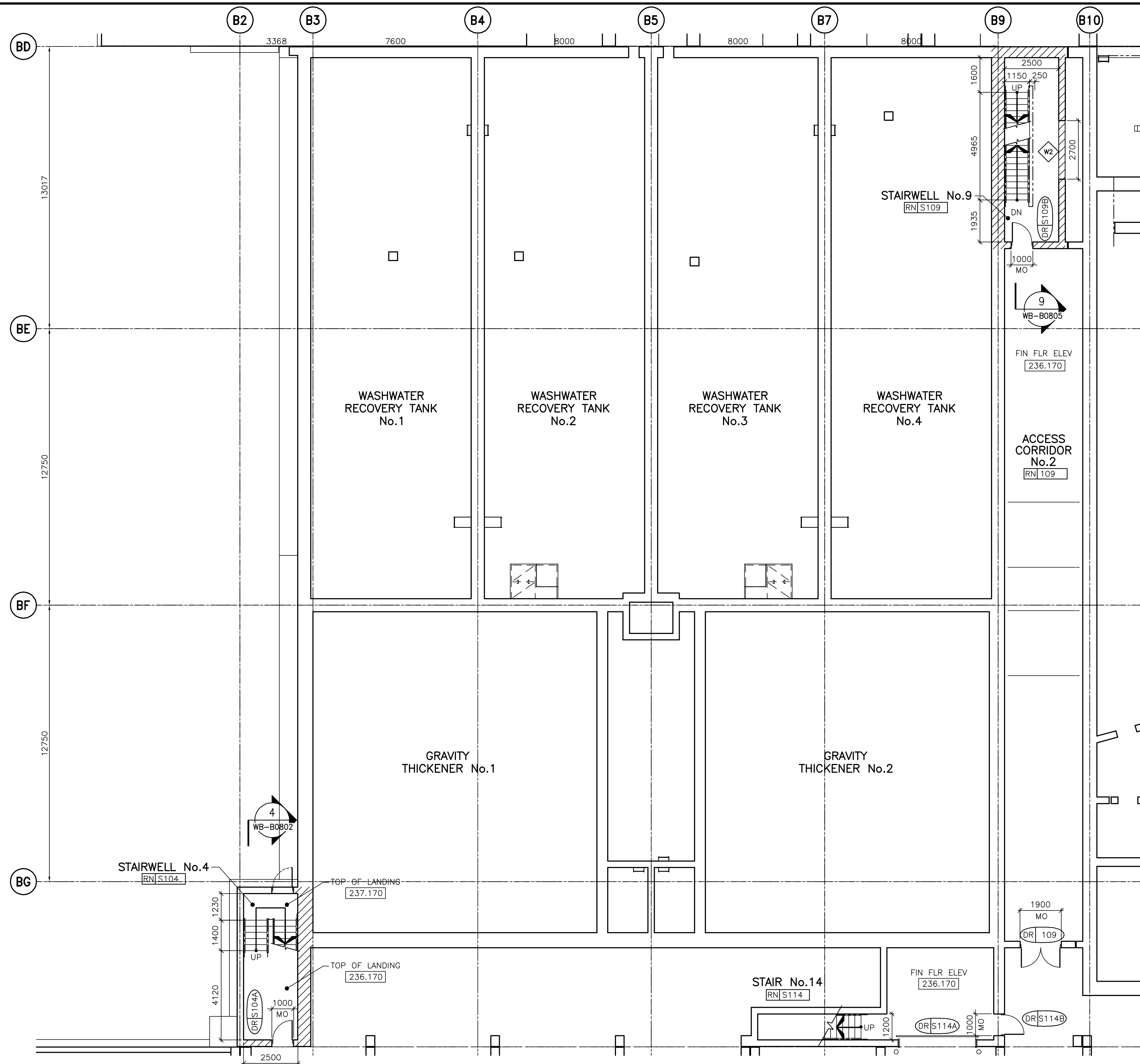
1 PARTIAL PLAN - RESIDUAL TANK AREA (FIRST FLOOR) WB-B0113 1:100
