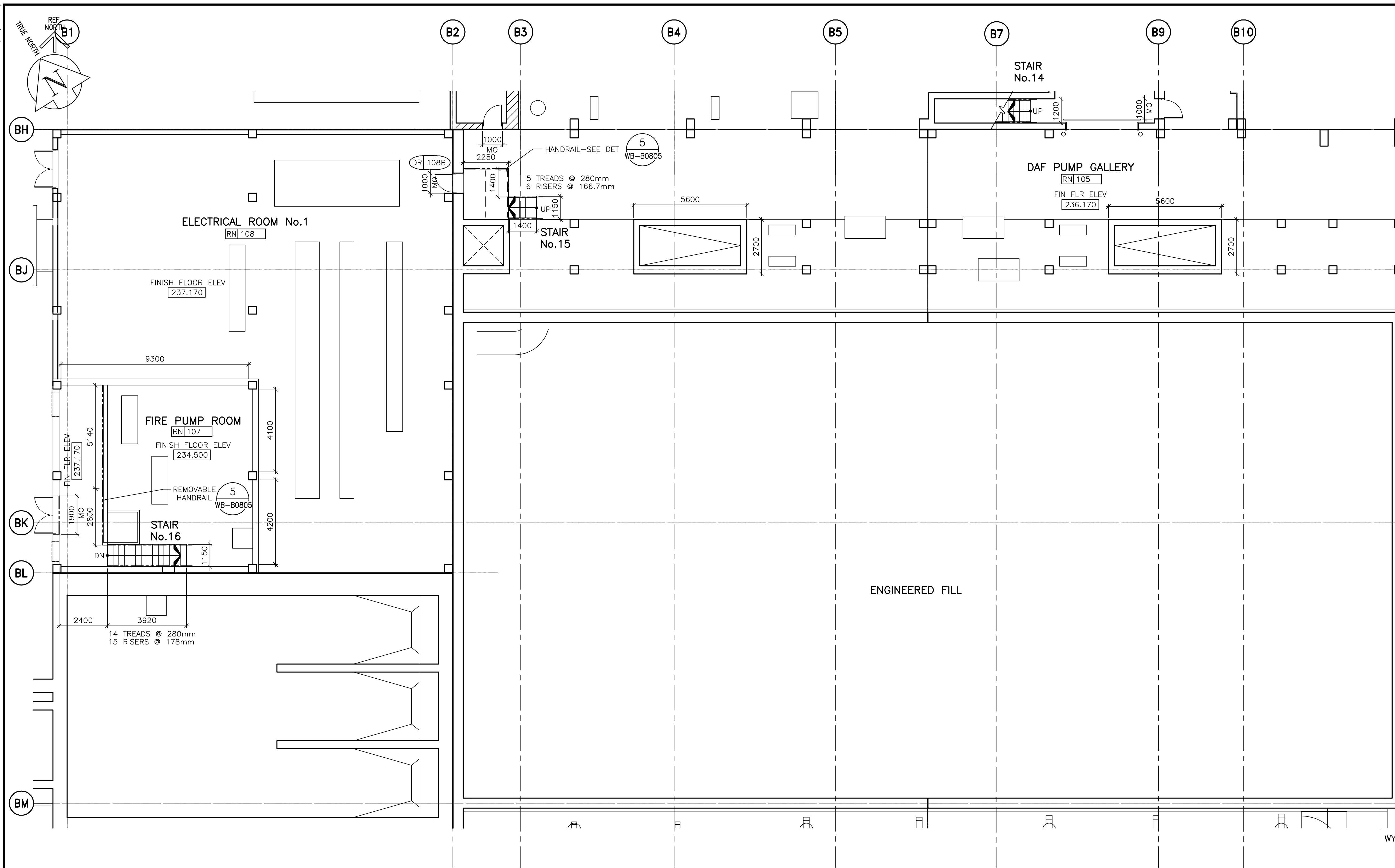
1 PARTIAL PLAN - DAF TANK, ELECTRICAL ROOM & FIRE PUMP ROOM (FIRST FLOOR) WB-B0116 1:100
