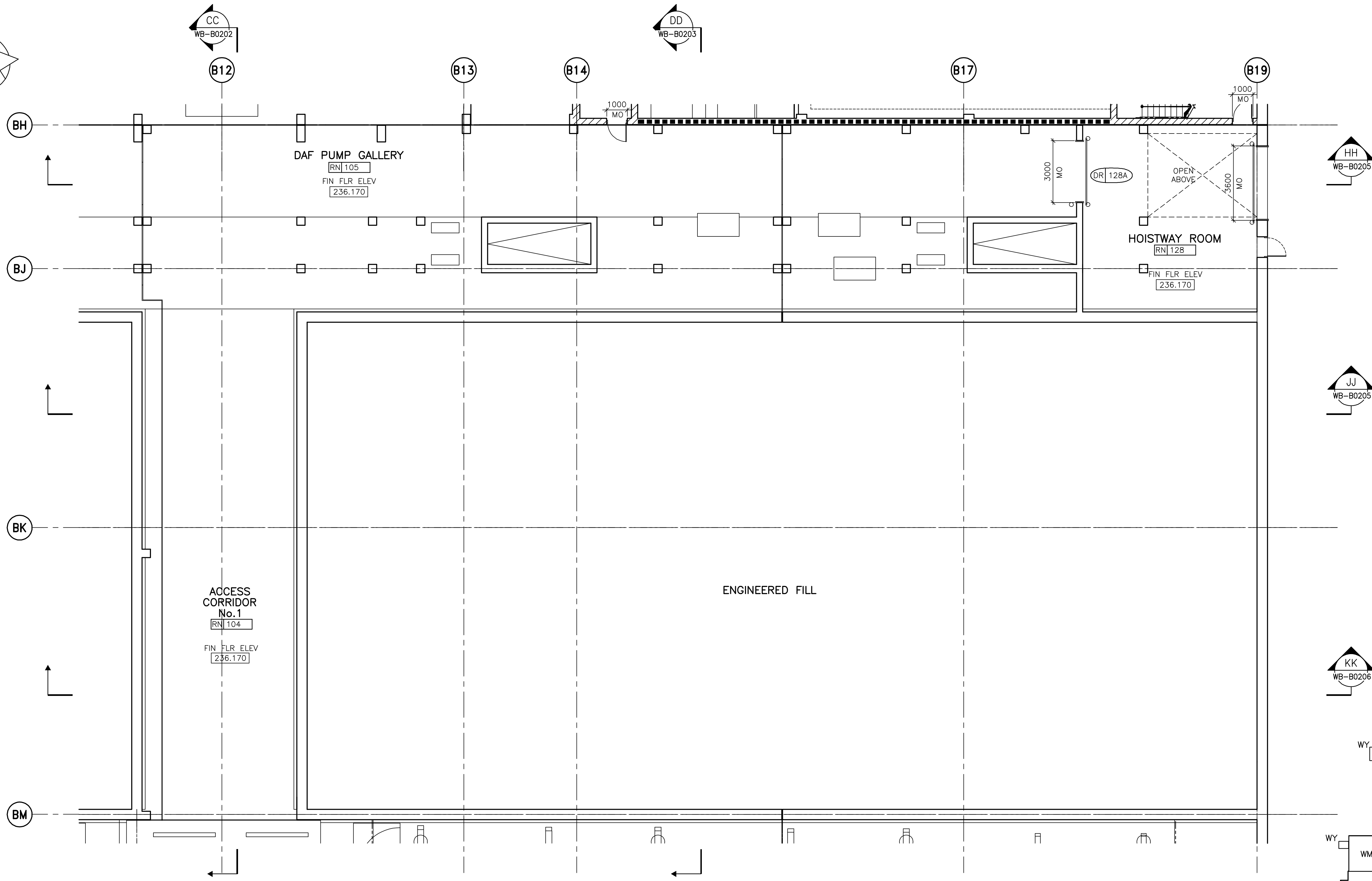
1 PARTIAL PLAN - DAF TANK PUMP GALLERY AND PIPE GALLERY AREA (FIRST FLOOR) WB-B0117 1:100
