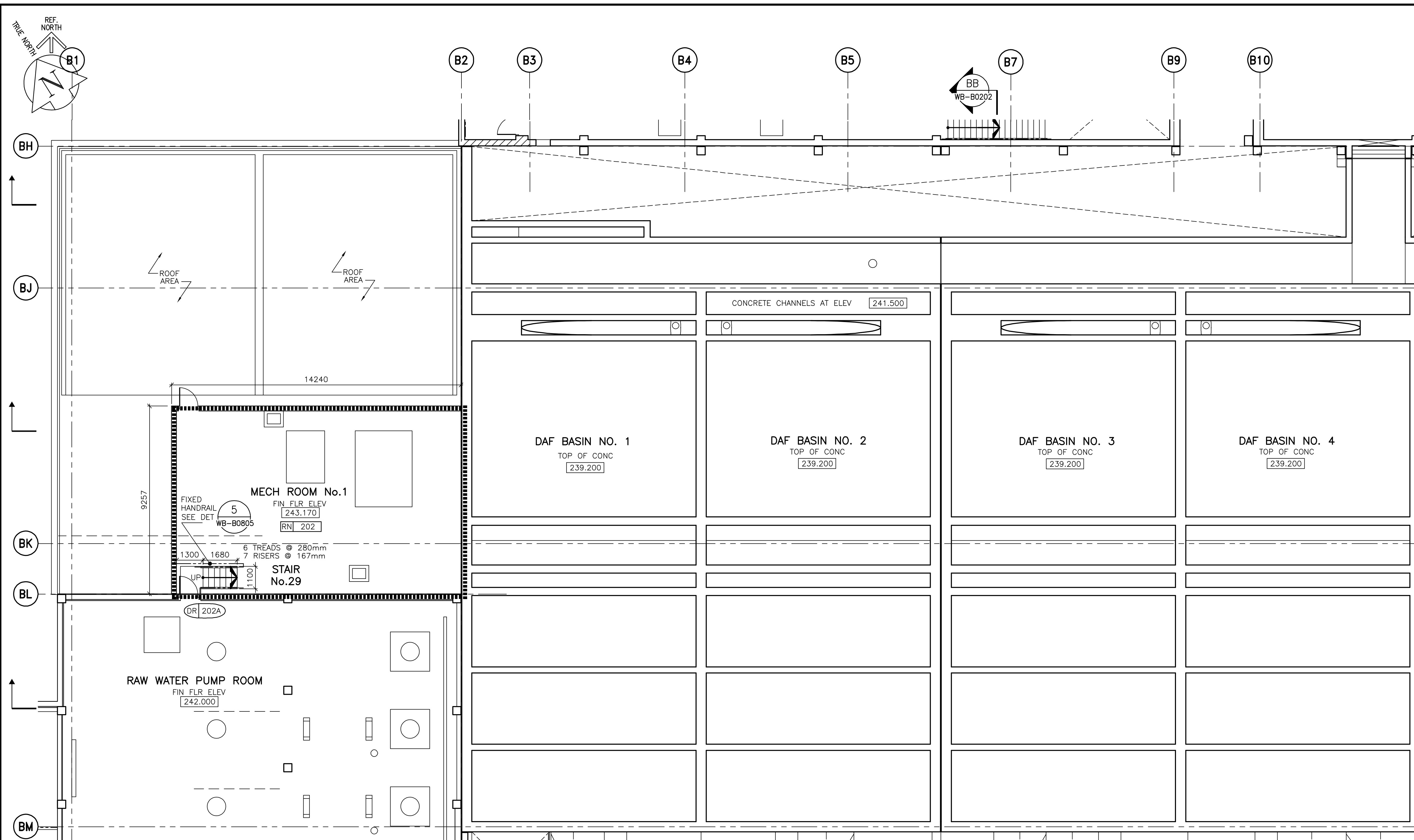
1 PARTIAL PLAN - DAF TANK & MECHANICAL RM NO. 1 AREA (SECOND FLOOR) WB-B0126 1:100
