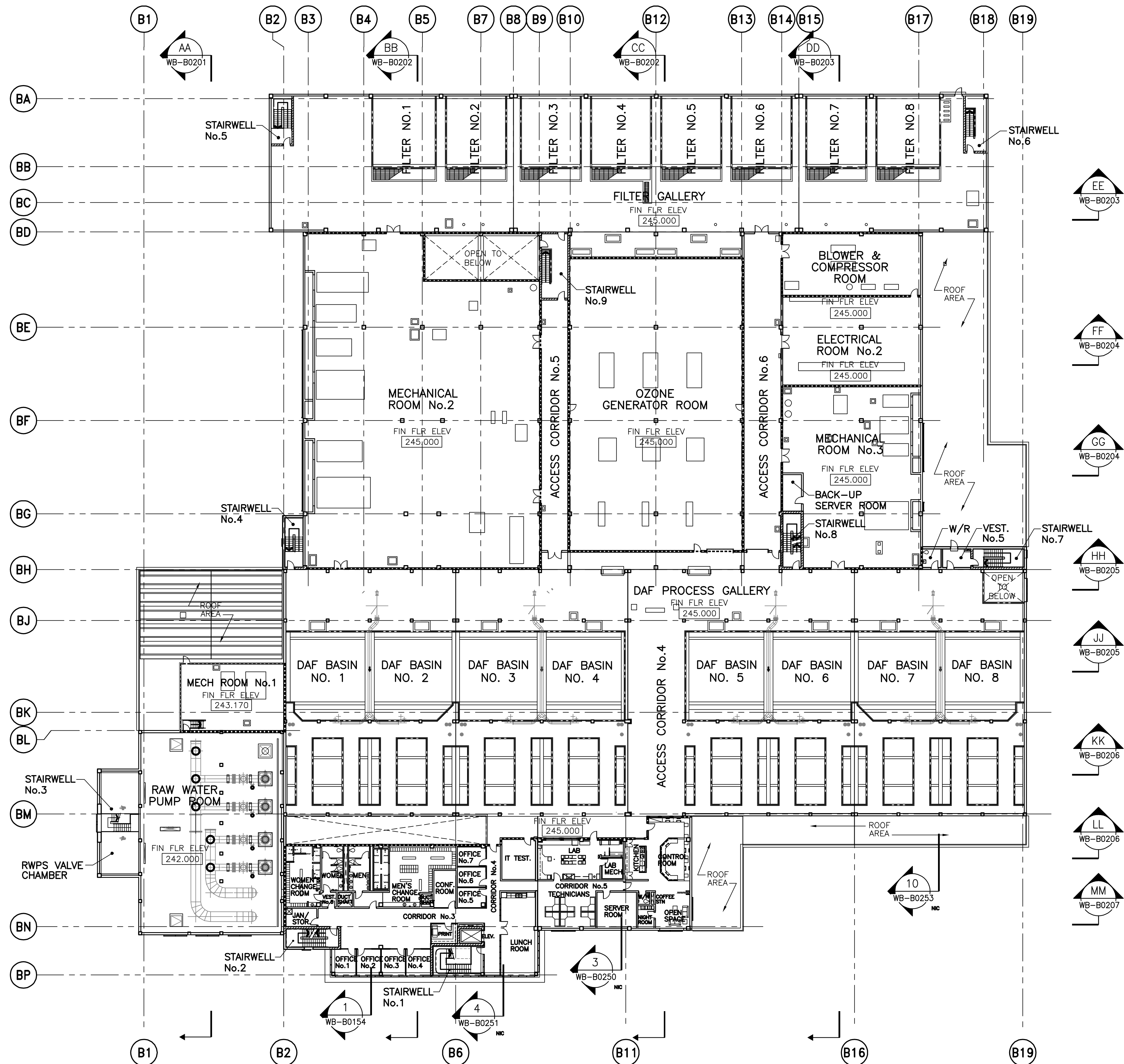
1 THIRD FLOOR PLAN WB-B0130 SCALE 1:300
