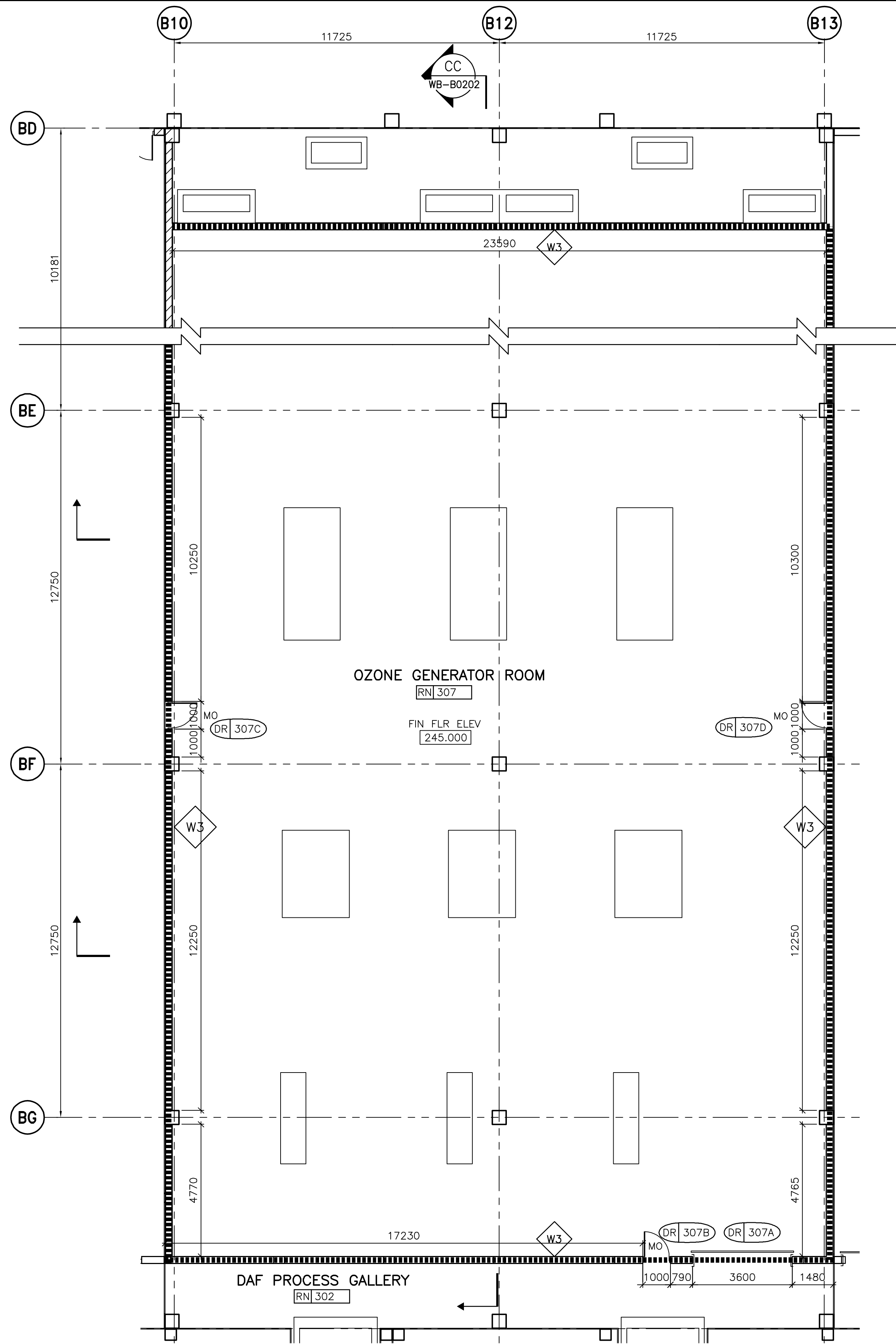
1 PARTIAL PLAN - OZONE GENERATOR ROOM (THIRD FLOOR) WB-B0134 1:100
