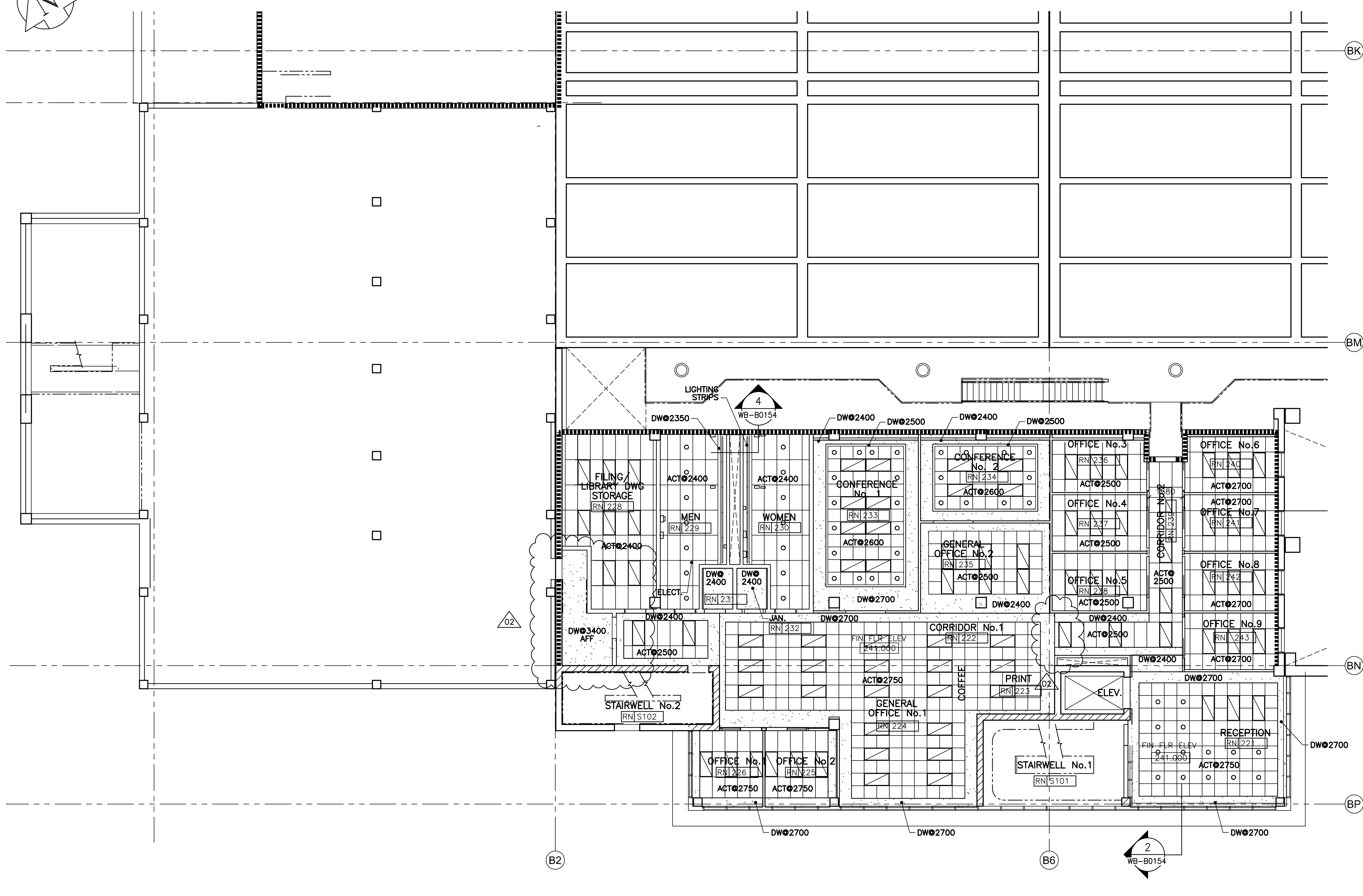
1 PARTIAL REFLECTED CEILING PLAN - ADMINISTRATION AREA (SECOND FLOOR) WB-B0152 1:100
