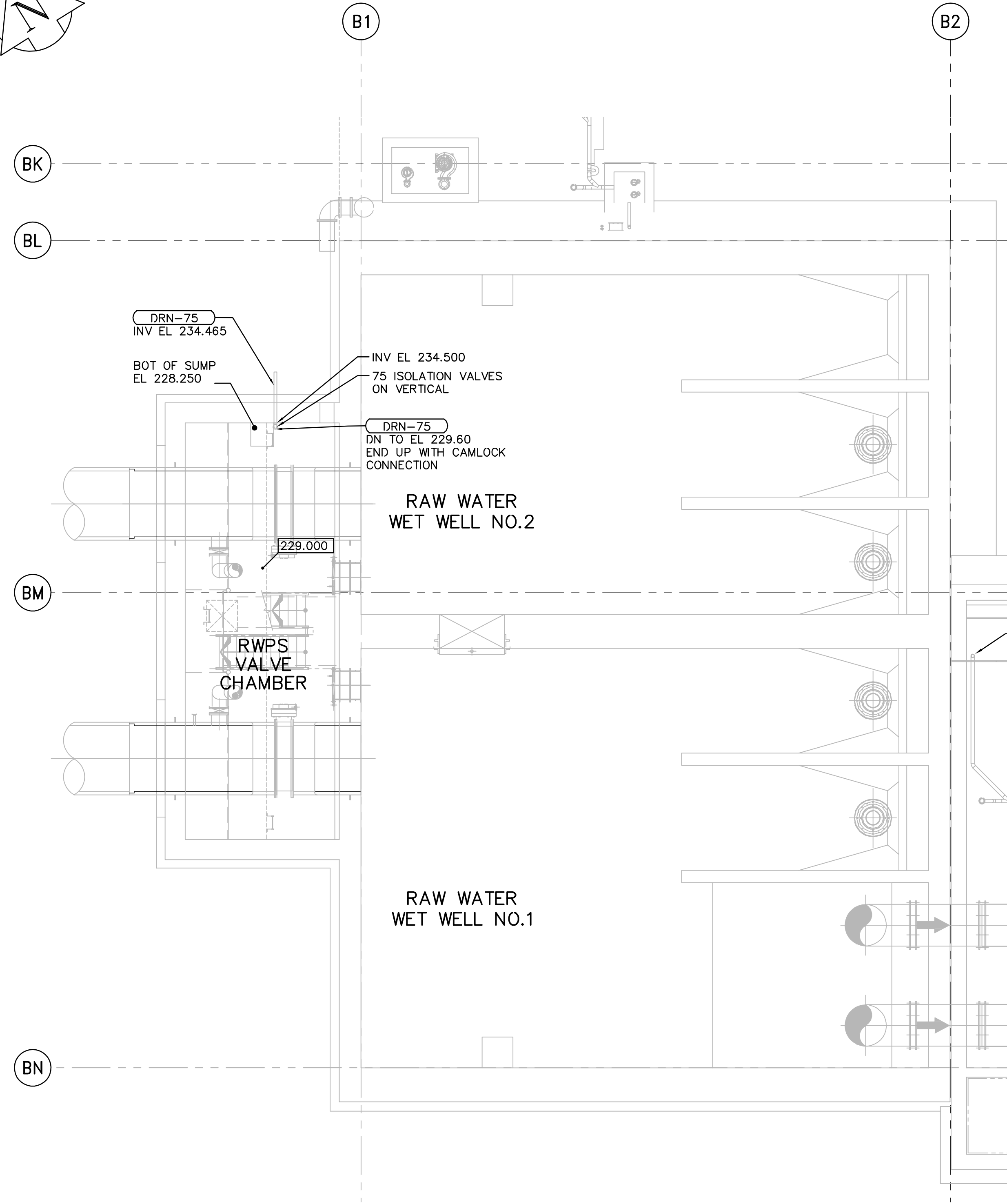
LOWER LEVEL PLAN 1:100
