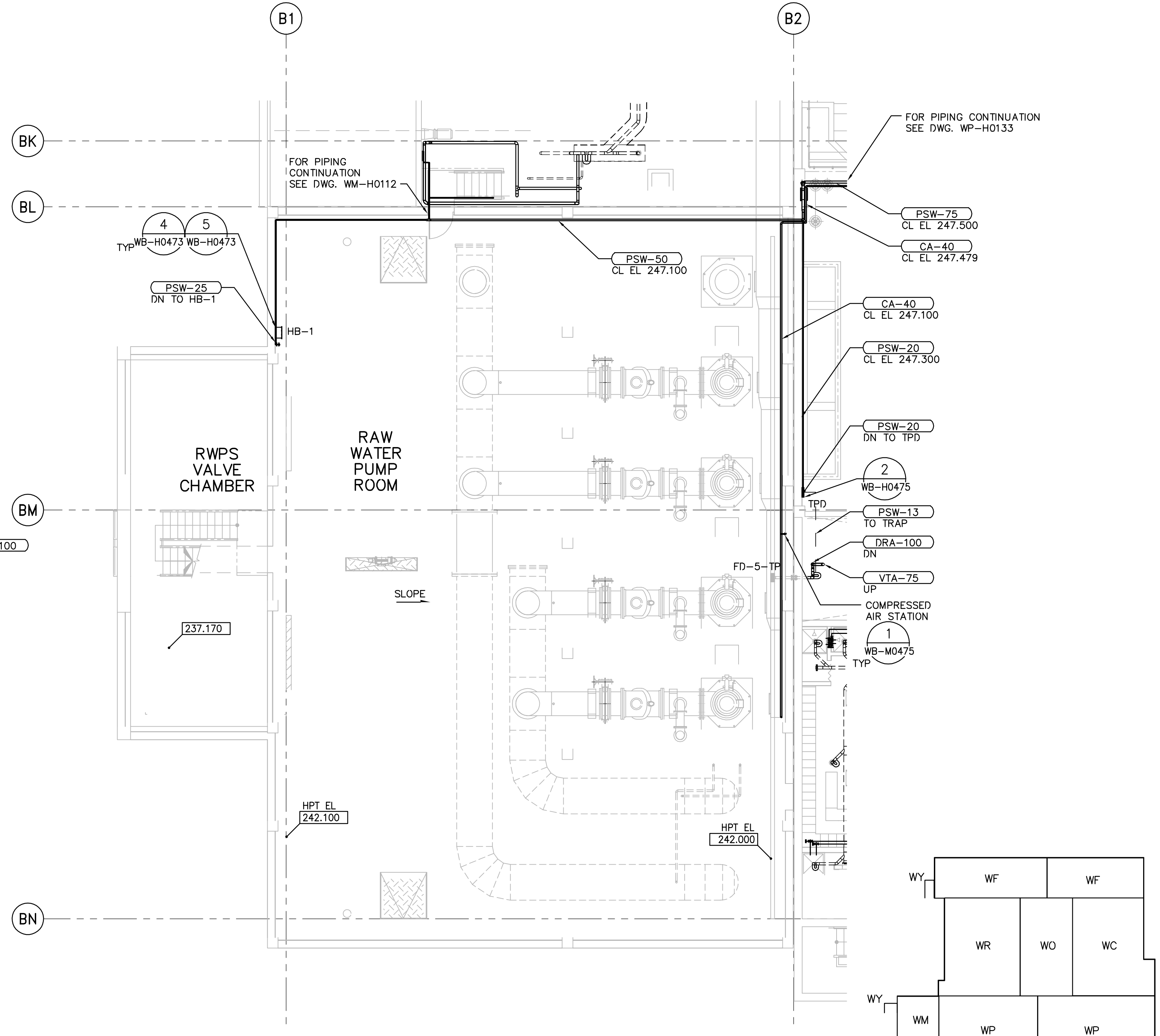
THIRD FLOOR PLAN 1:100
