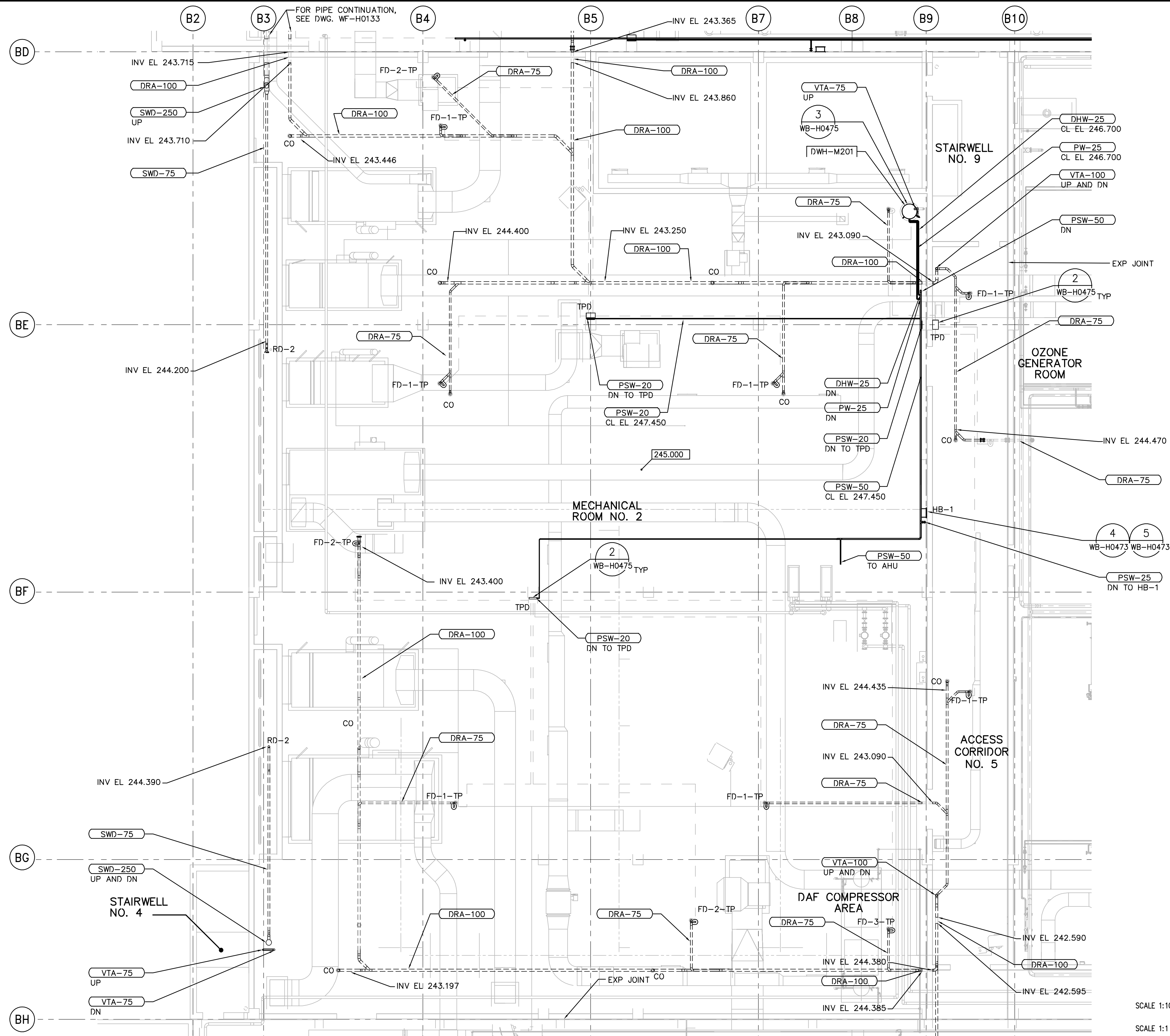
THIRD FLOOR PLAN 1:100
