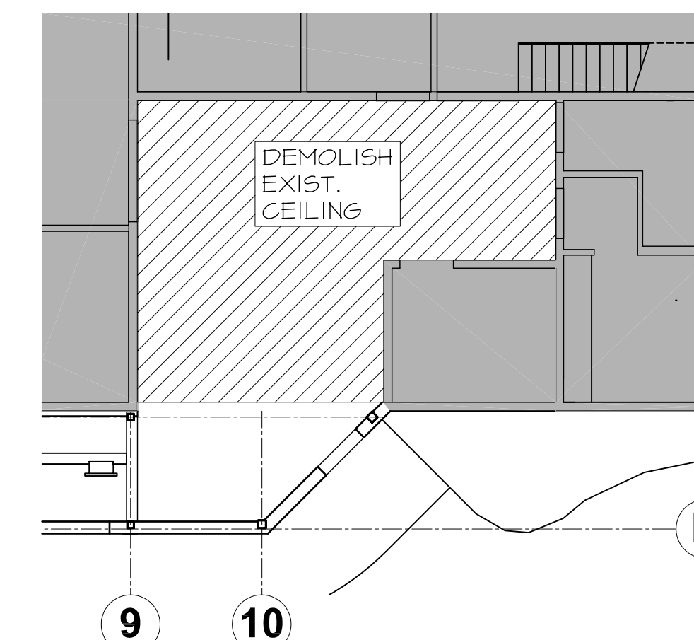
3 CEILING DEMOLITION PLAN 4.1 4.1 1:100
