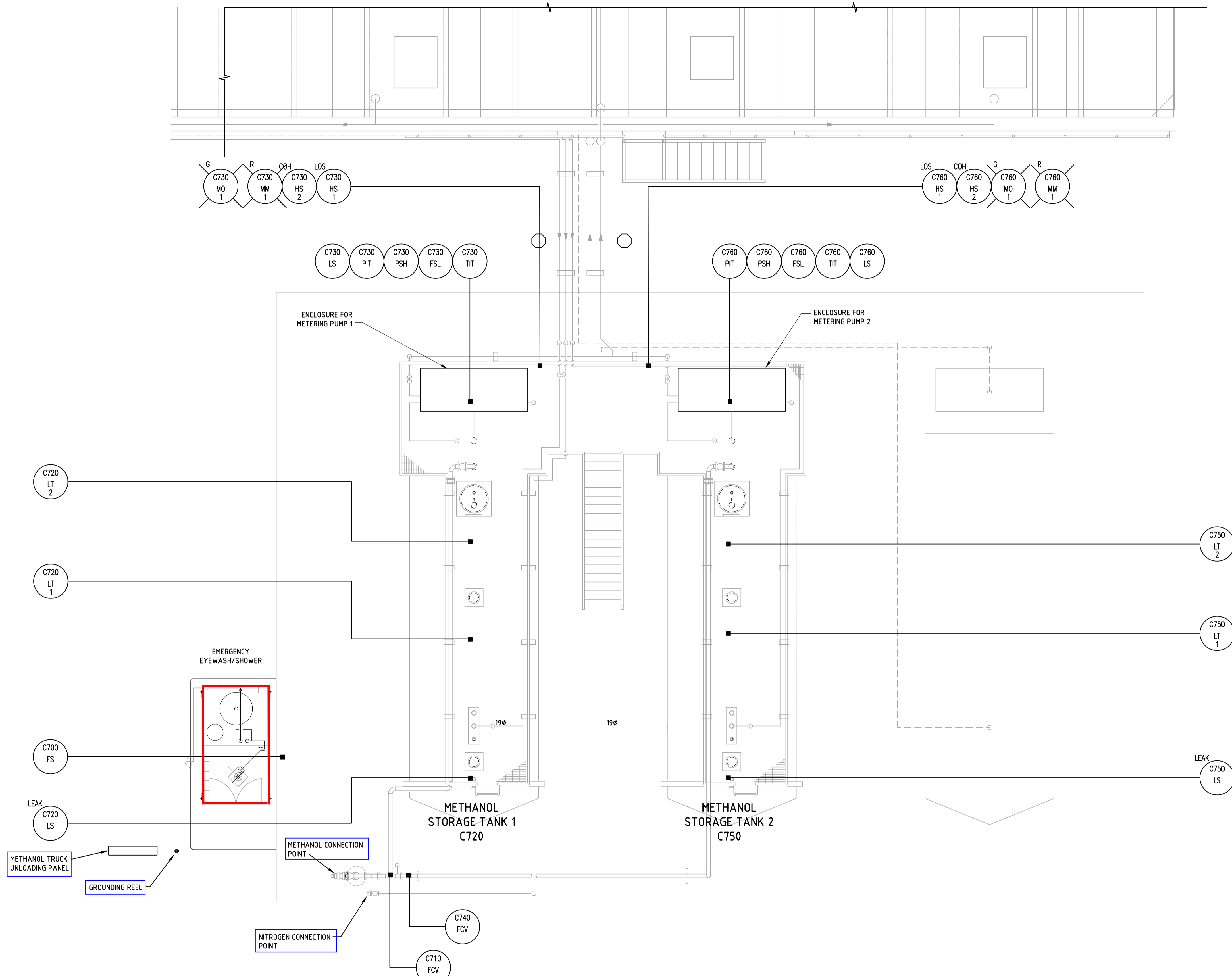
1 METHANOL DOSING TANKS INSTRUMENT PLAN SCALE 1:50
