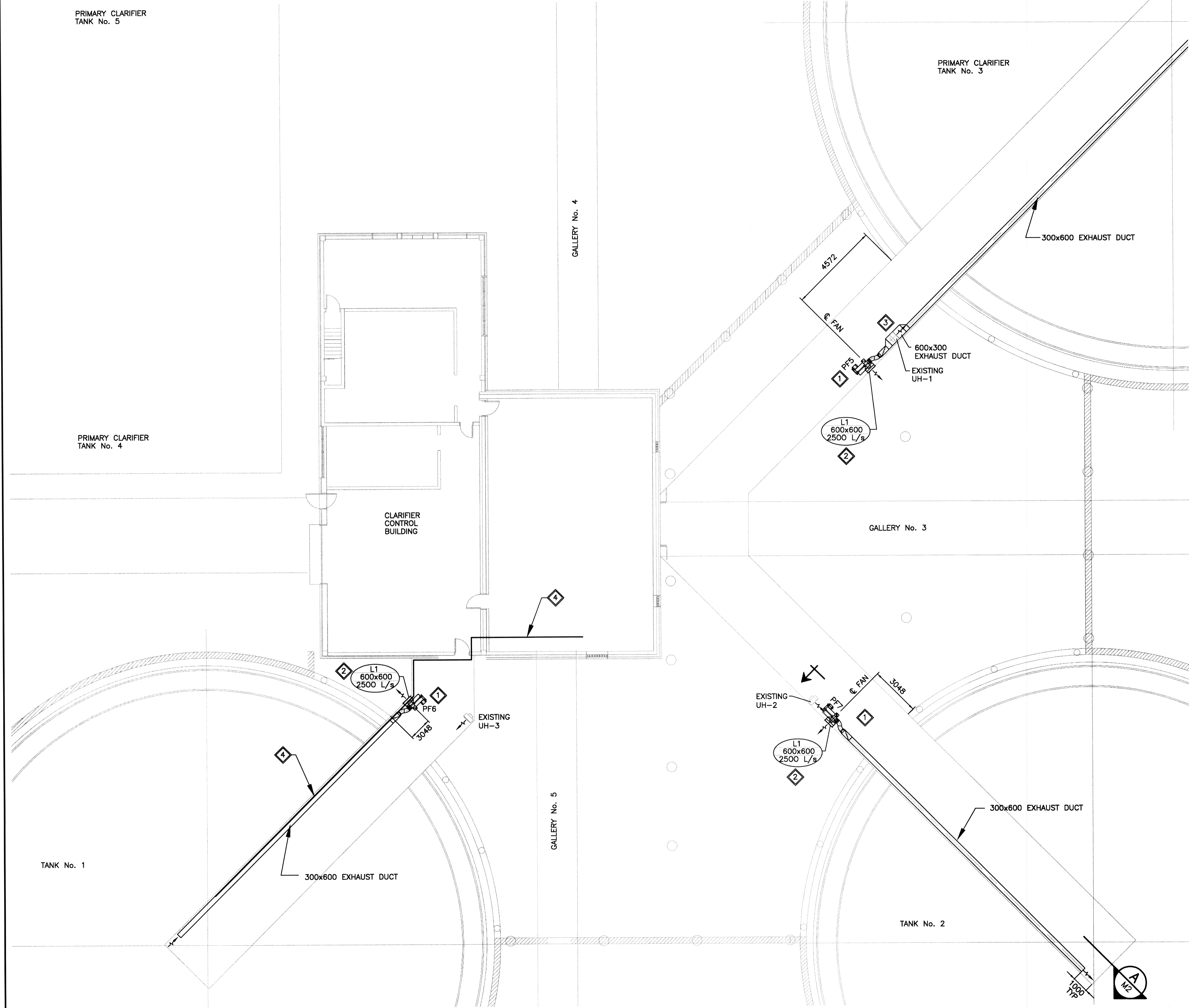
1 PLAN OF WALKWAY ENCLOSURE VENTILATION SCALE: 1:125mm
