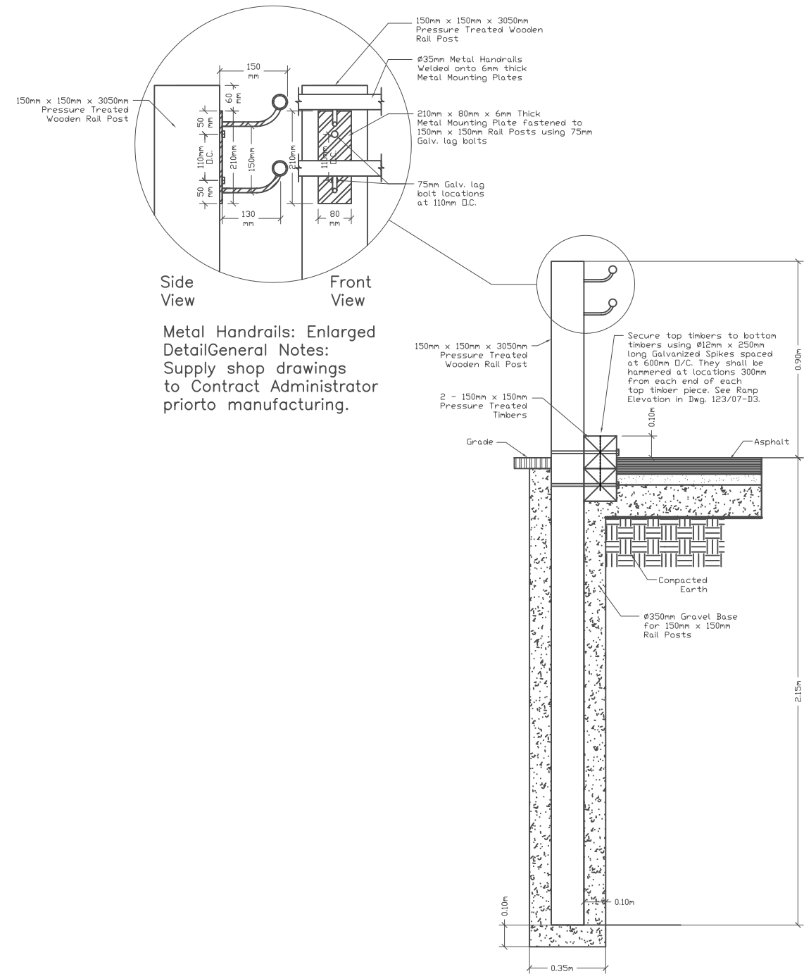
3 D2 Handrail Post & Metal Rails Detail
