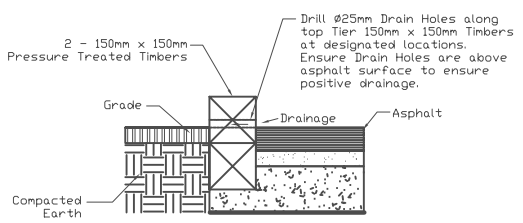
2 D2 Drain Hole Detail
