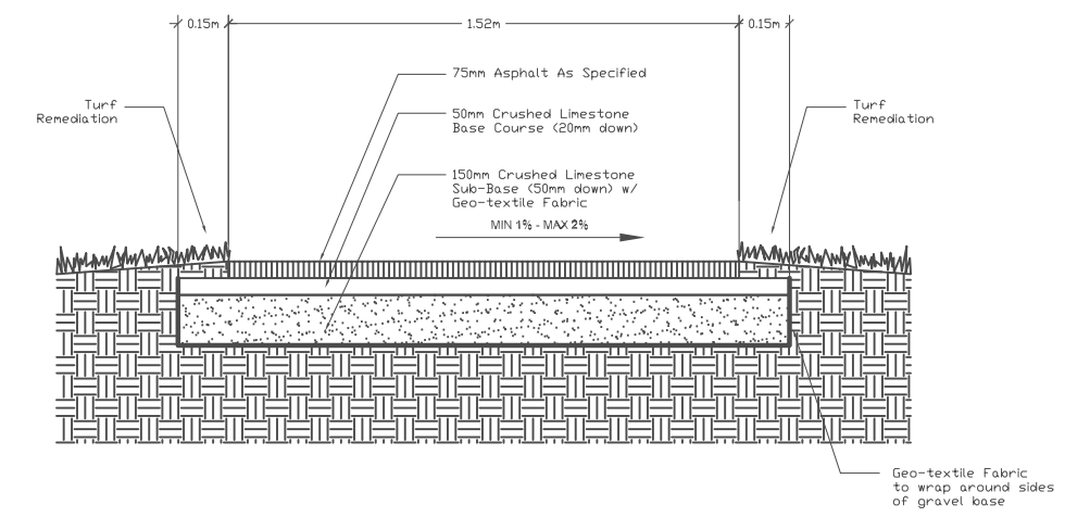
4 D2 Asphalt Path Detail
