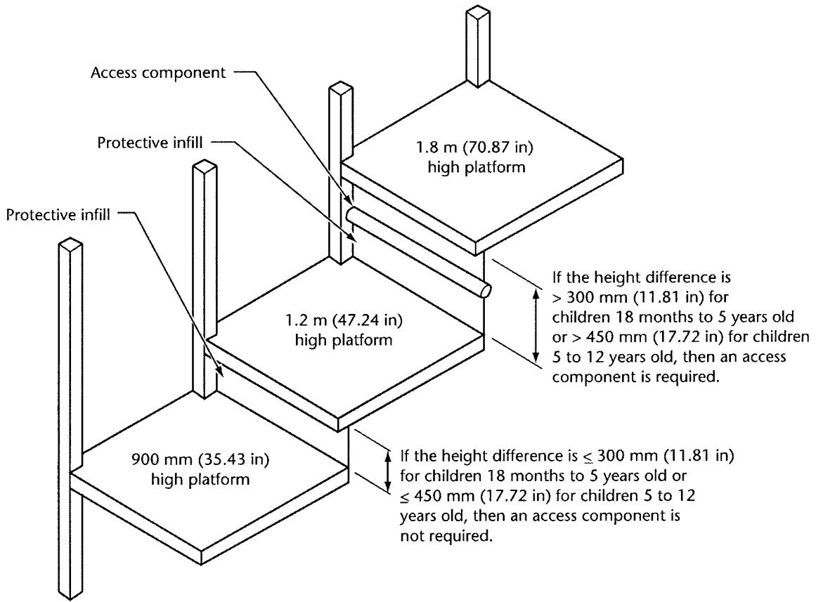
Figure 21 Adjacent platform requirements
