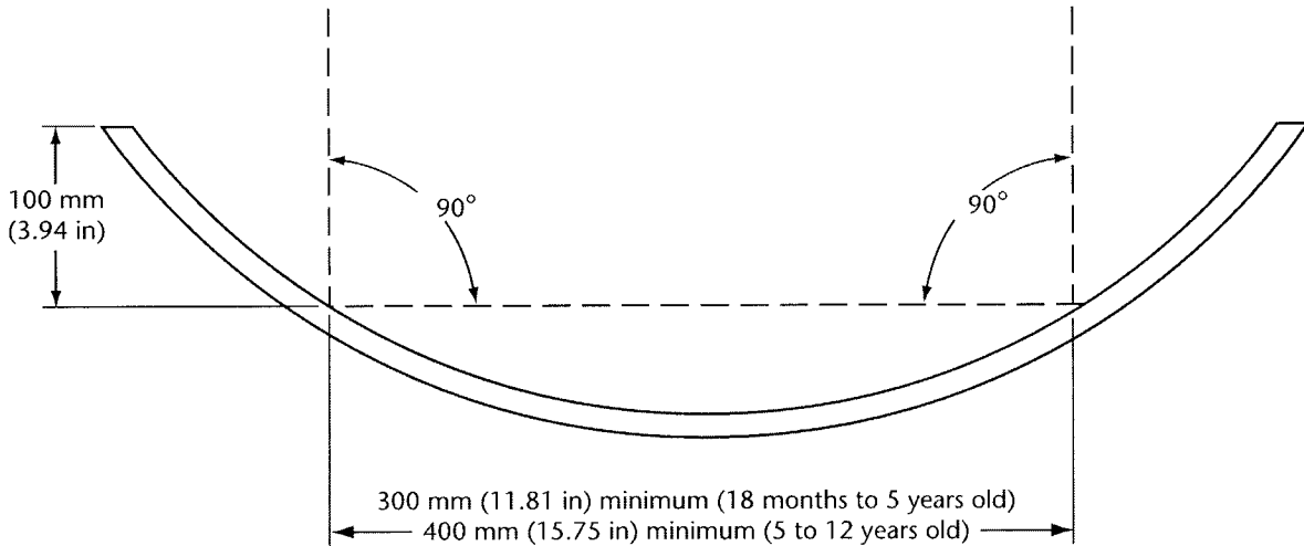
Figure 36 Details of the slide cross-section
