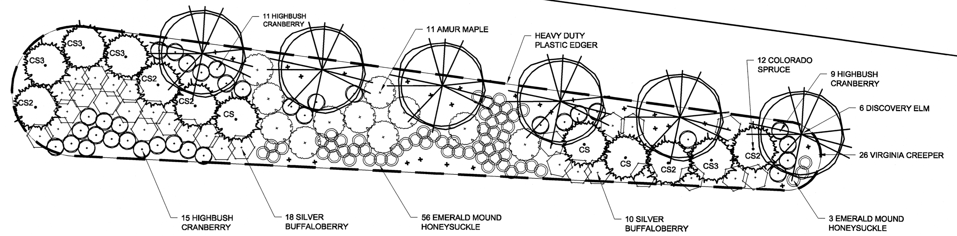
PLANTING DETAIL 11 SHRUB BED ENLARGEMENT SCALE 1:250 0 2.5 5 7.5 m
