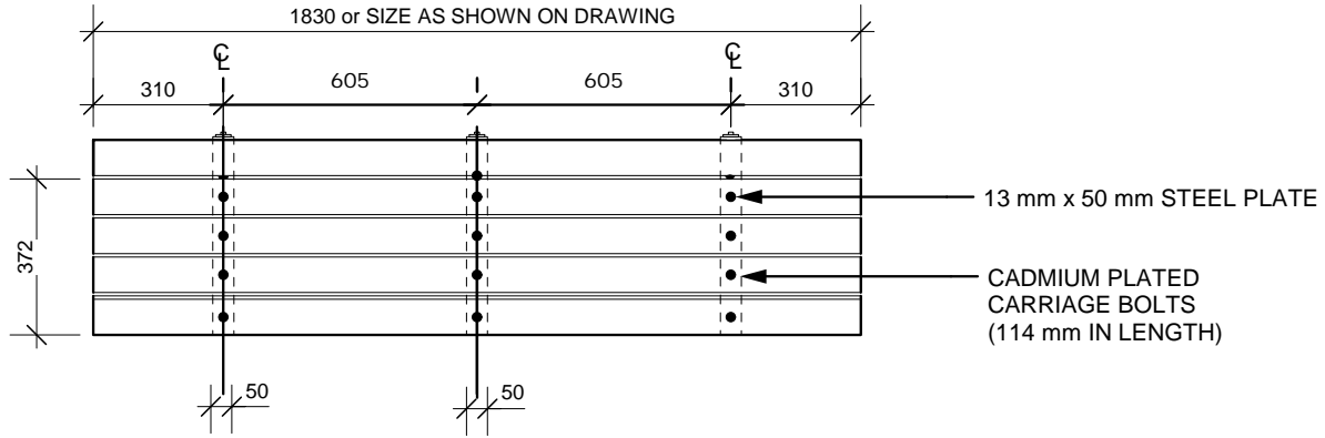
PLAN VIEW
