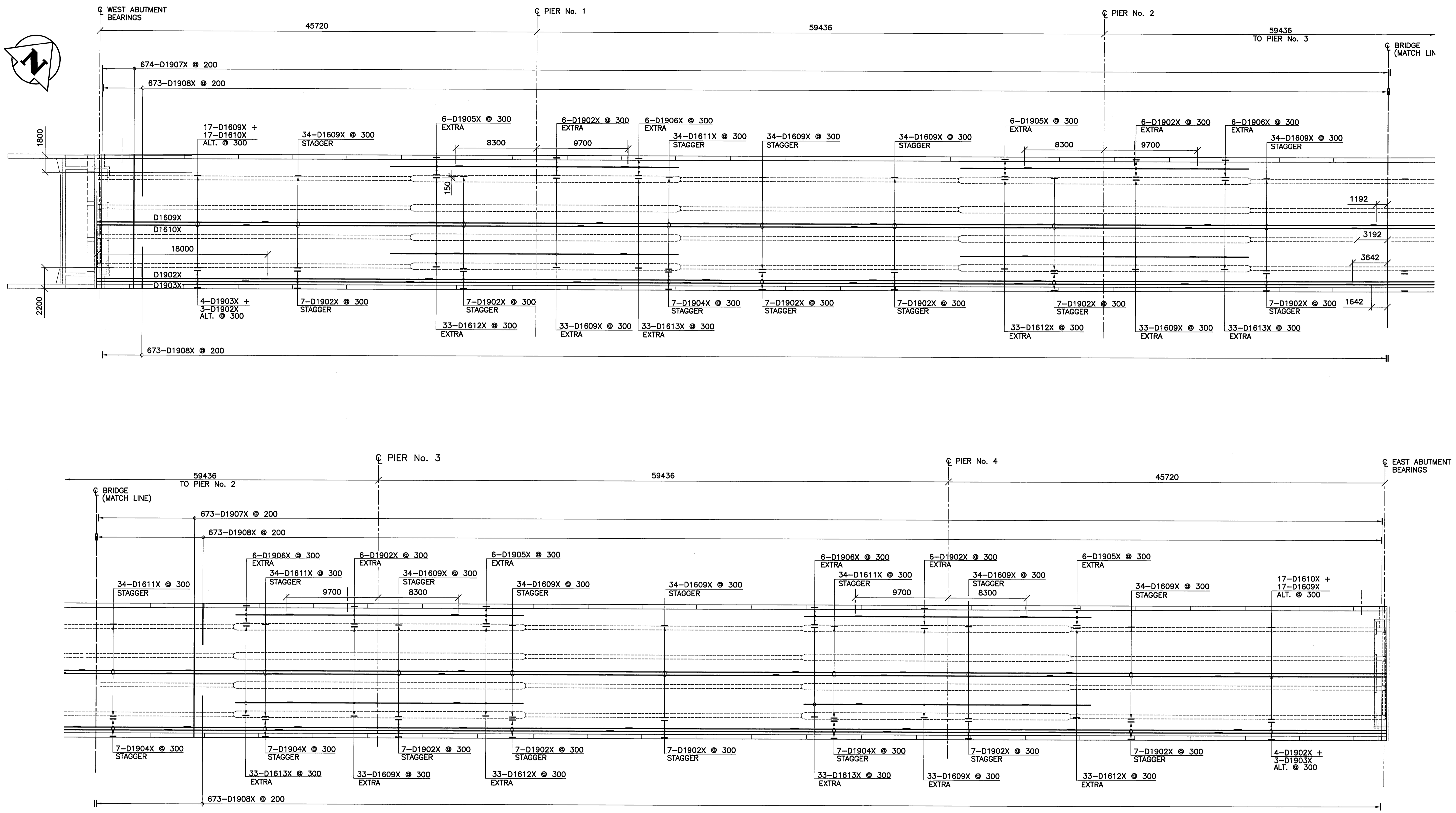
1 DECK TOP REINFORCING PLAN 1 : 200
