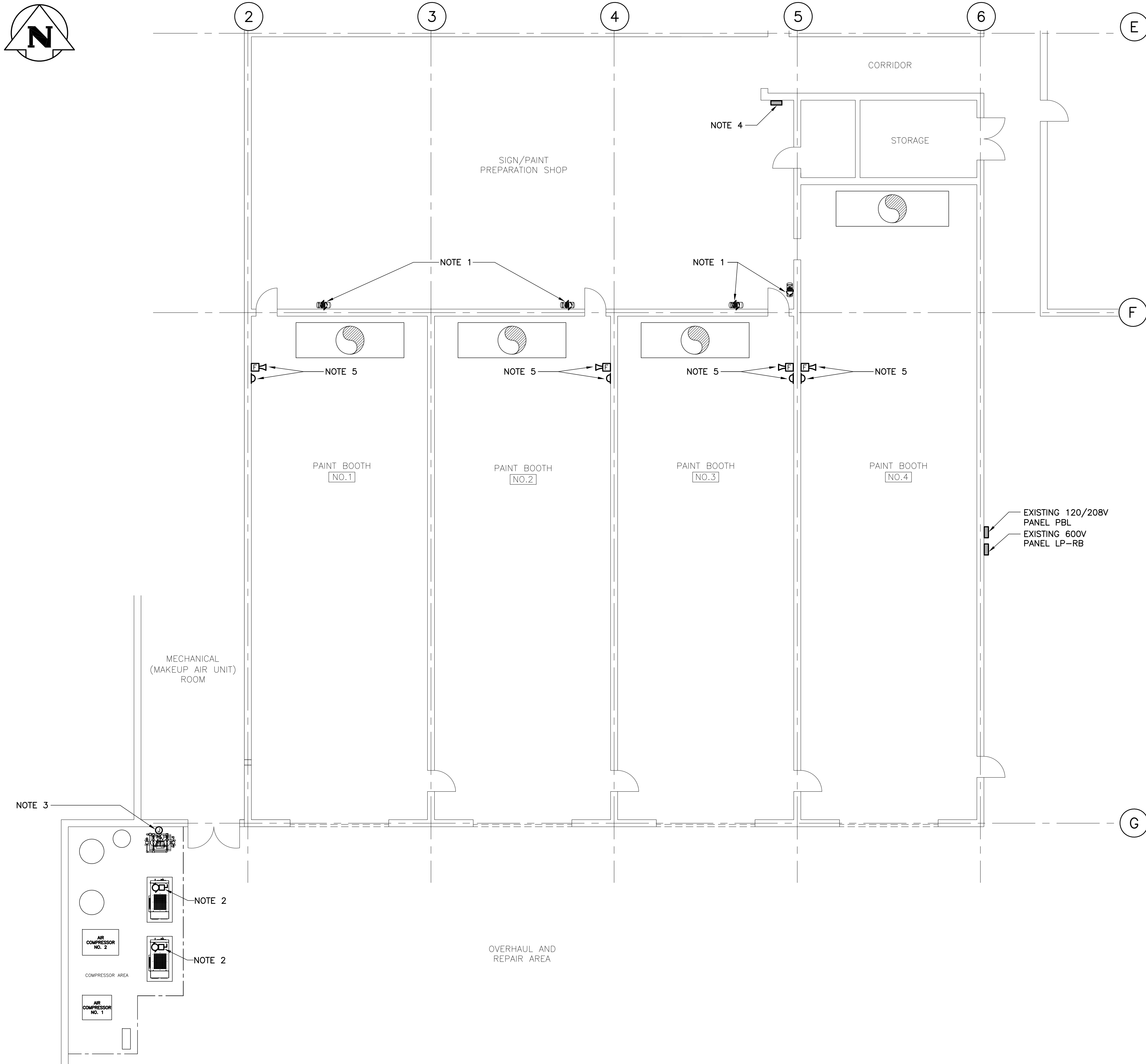
1 PARTIAL MAIN FLOOR PLAN - ELECTRICAL LAYOUT 1/8" = 1'-0"
