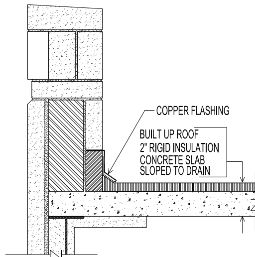
PARAPET DETAIL (EXISTING) SCALE: NTS
