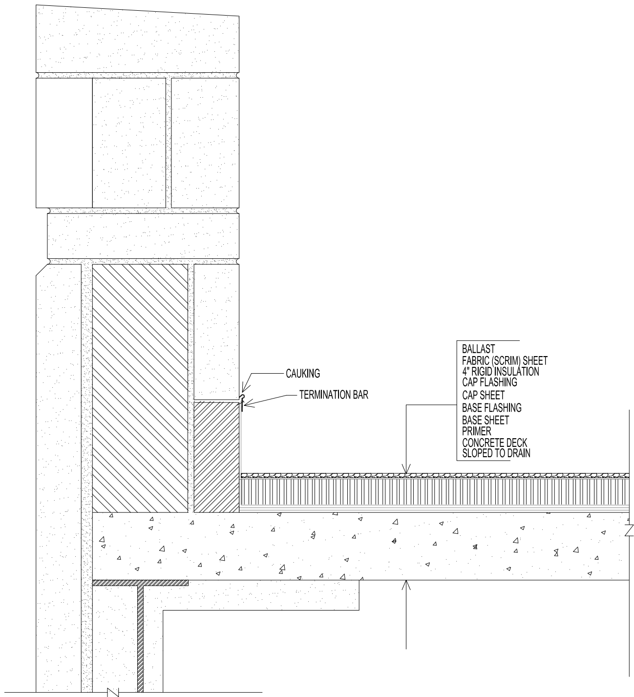
TYPICAL NEW EDGE DETAIL SCALE: NTS
