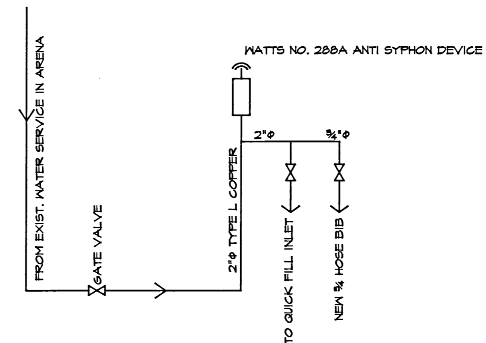
SUPPLY SCHEMATIC
