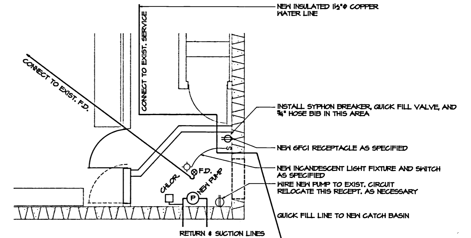
PUMP ROOM LAYOUT SCALE: 1/4"=1'0"
