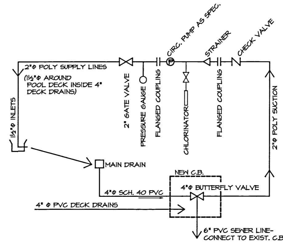
POOL SYSTEM SCHEMATIC
