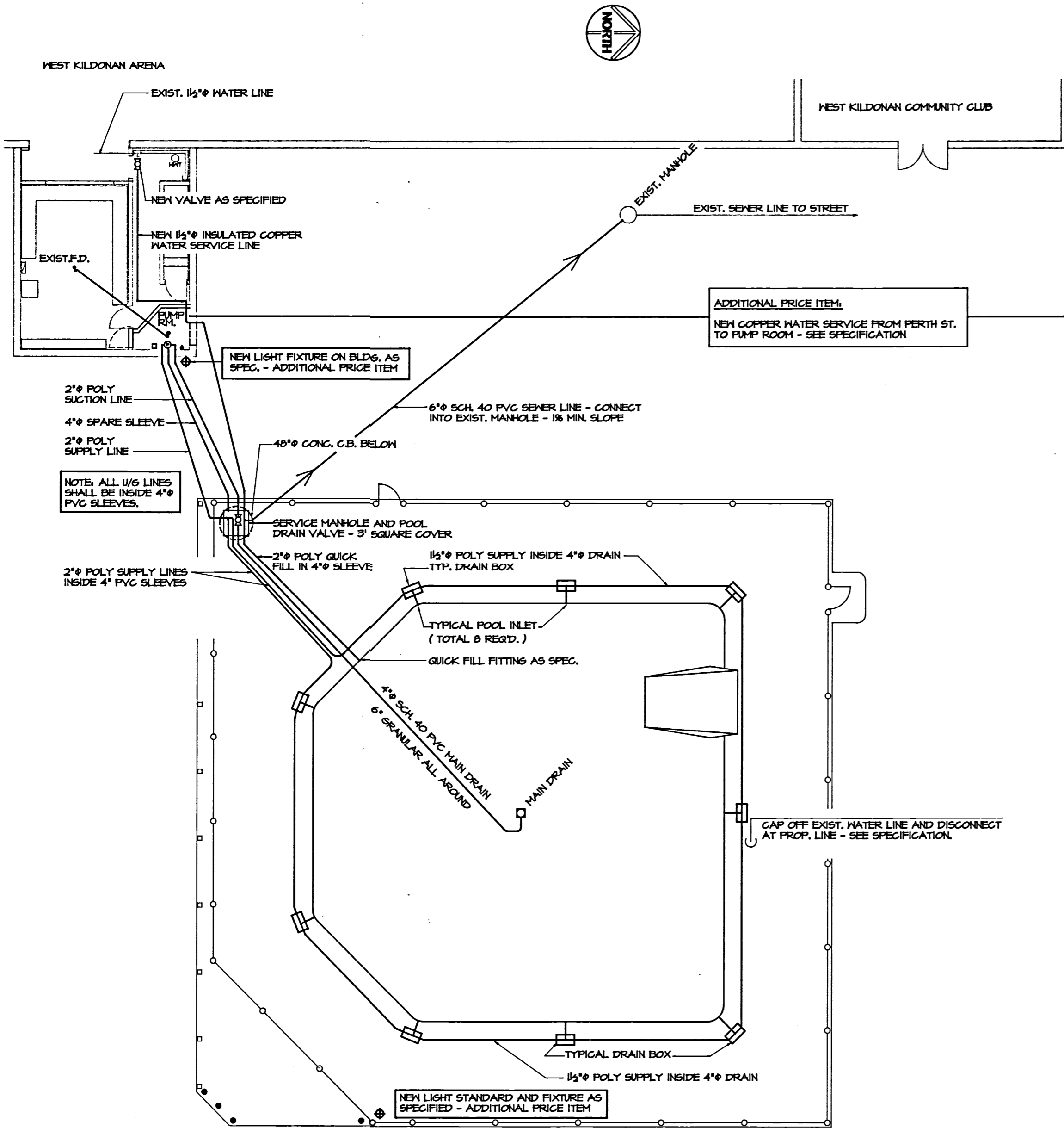
PIPING LAYOUT SCALE: 3/32"=1'0"
