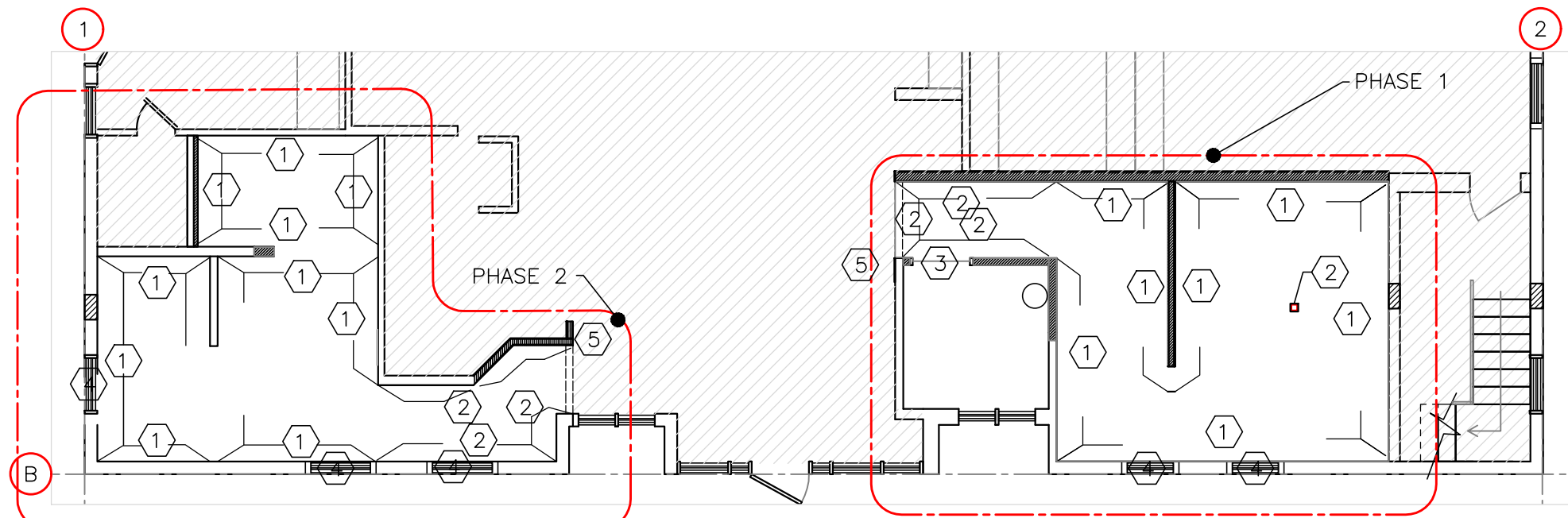
Wall Finish Plan
