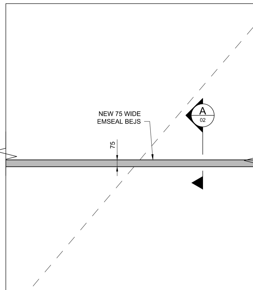
2 DETAIL 1:20
