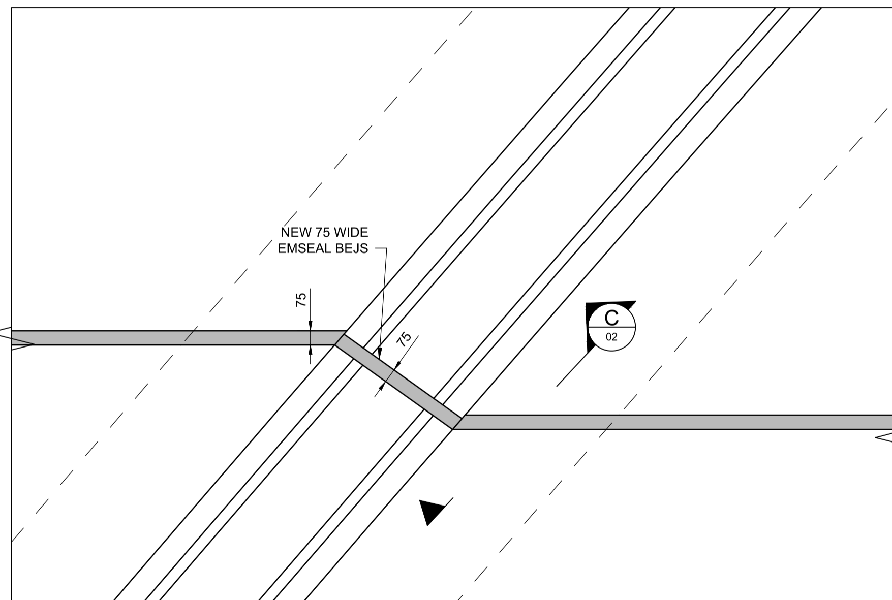
3 DETAIL 1:20
