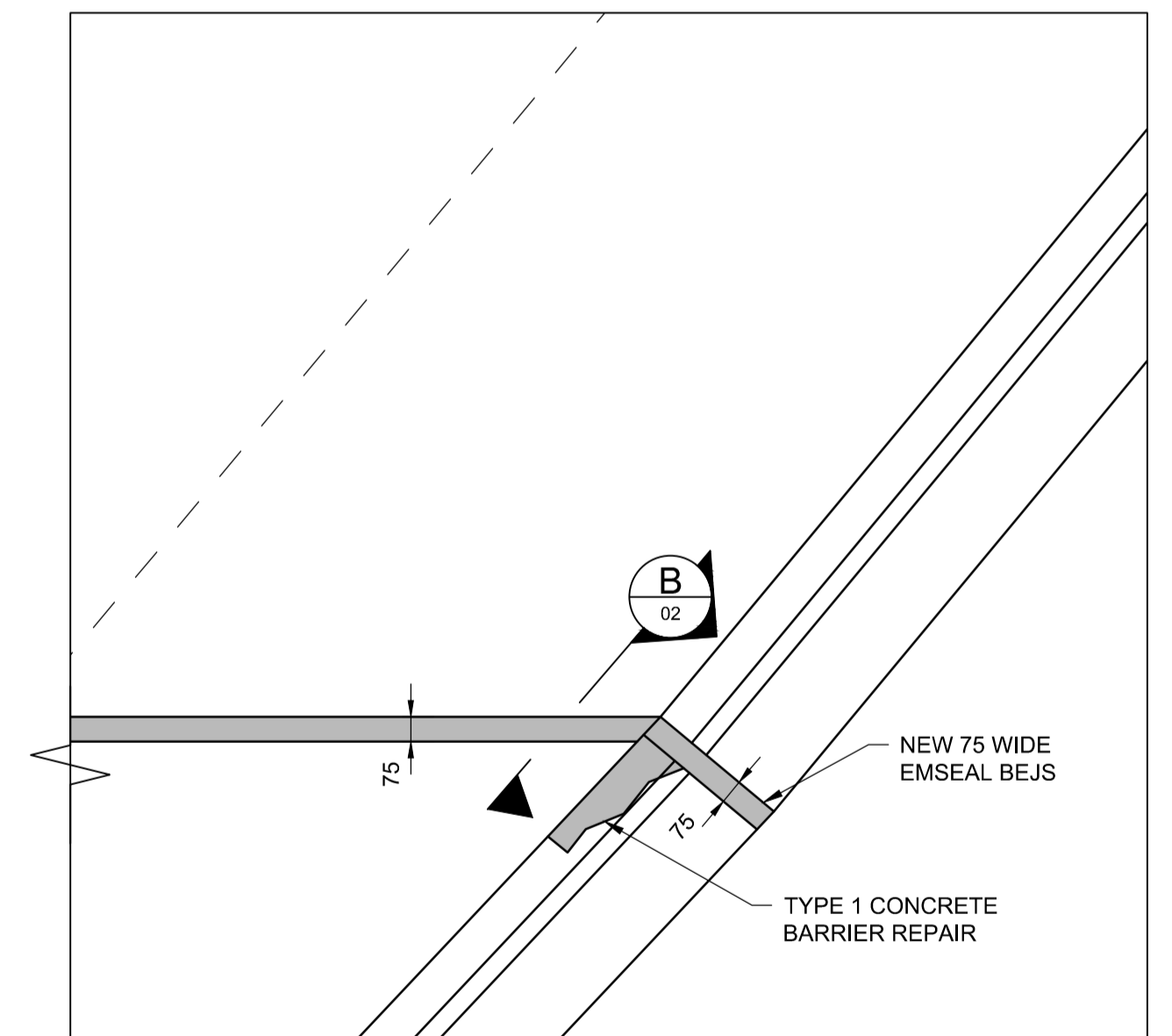
4 DETAIL 1:20
