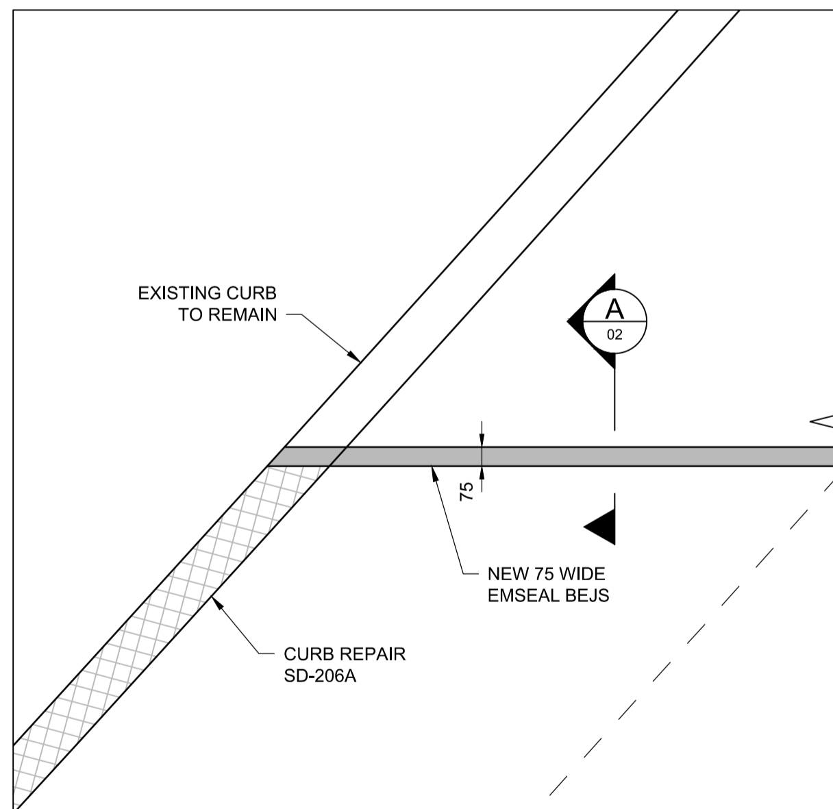
1 DETAIL 1:20
