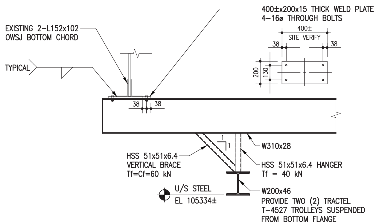
3 SECTION S2.3 | S2.4 1:20
