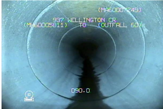
Photo 1: Approx. Sta. 1+90 looking d/s
