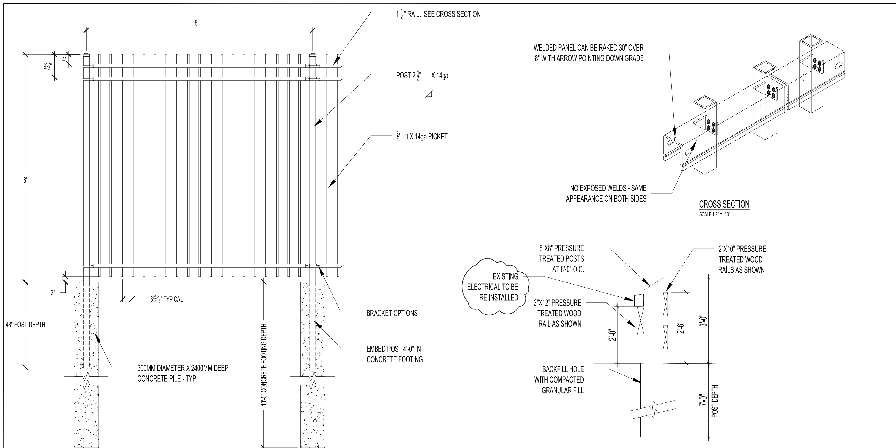
2 A2 LIGHT PROOF HEADLIGHT FENCE DETAIL SCALE 1/2" = 1'-0"
